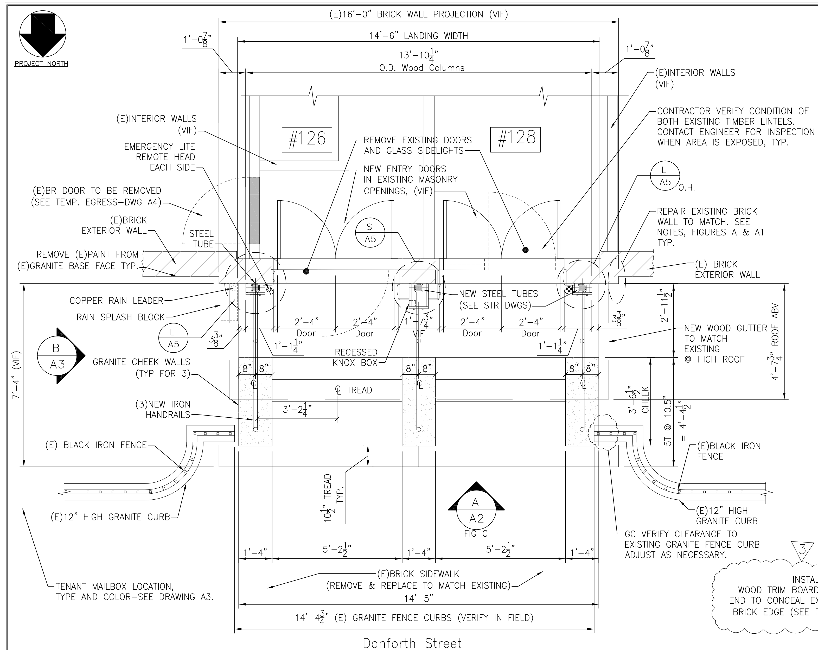
FRONT ENTRY PLAN SCALE: 1/2 = 1'-0"
