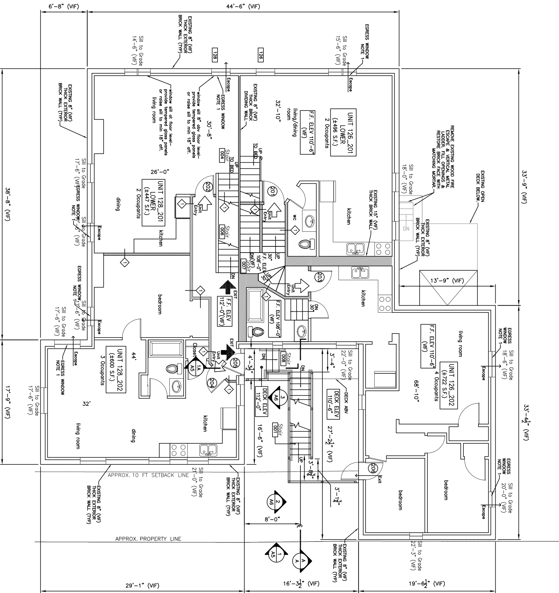
FLOOR 2 PLAN
