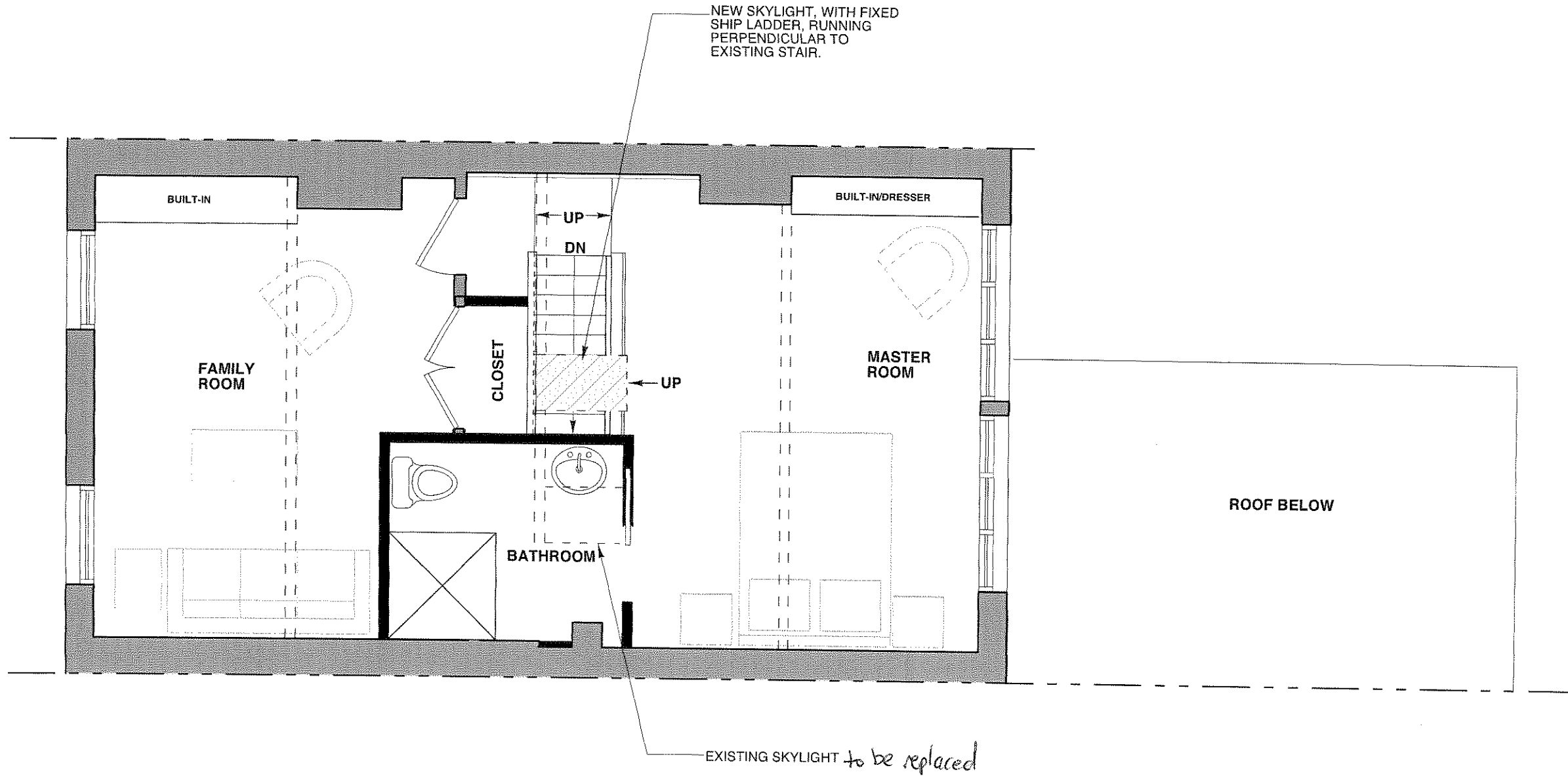
1 THIRD FLOOR PLAN OPTION B SCALE: 1/4" = 1'-0"
