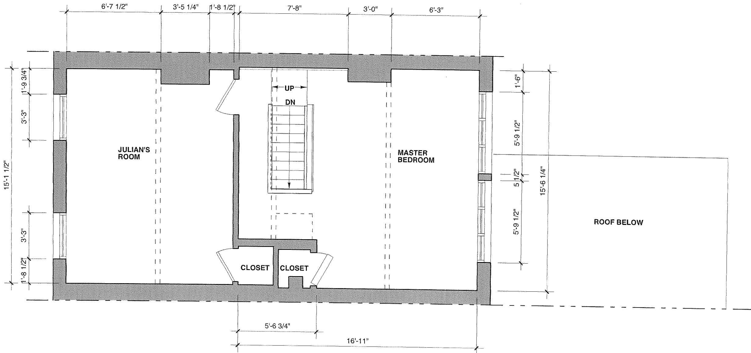
1 THIRD FLOOR PLAN SCALE: 1/4" = 1'-0"
