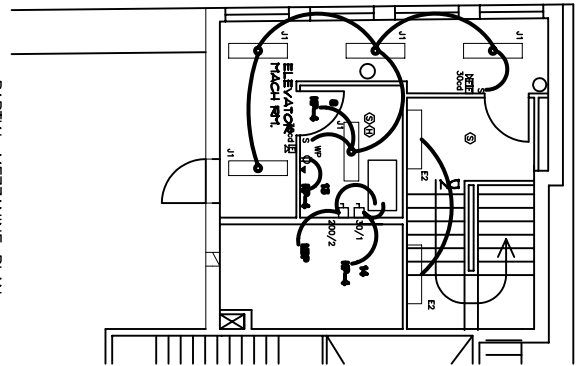
PARTIAL MEZZANINE PLAN 1/4" = 1'-0"
