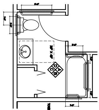
2 BEDROOM ACCESSIBLE UNITS NO.202 & 203
