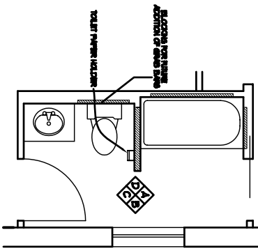
1 BEDROOM UNIT NOS 209 & 309 (ADAPTABLE)
