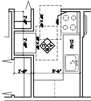
1 BEDROOM ACCESSIBLE UNIT NO. 401
