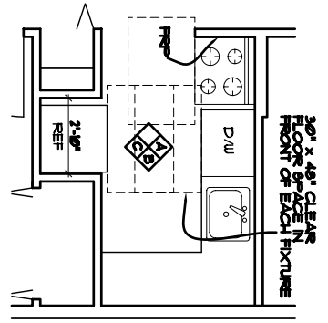
1 BEDROOM UNIT NOS 201 & 301
