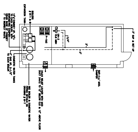
BASEMENT PLAN
