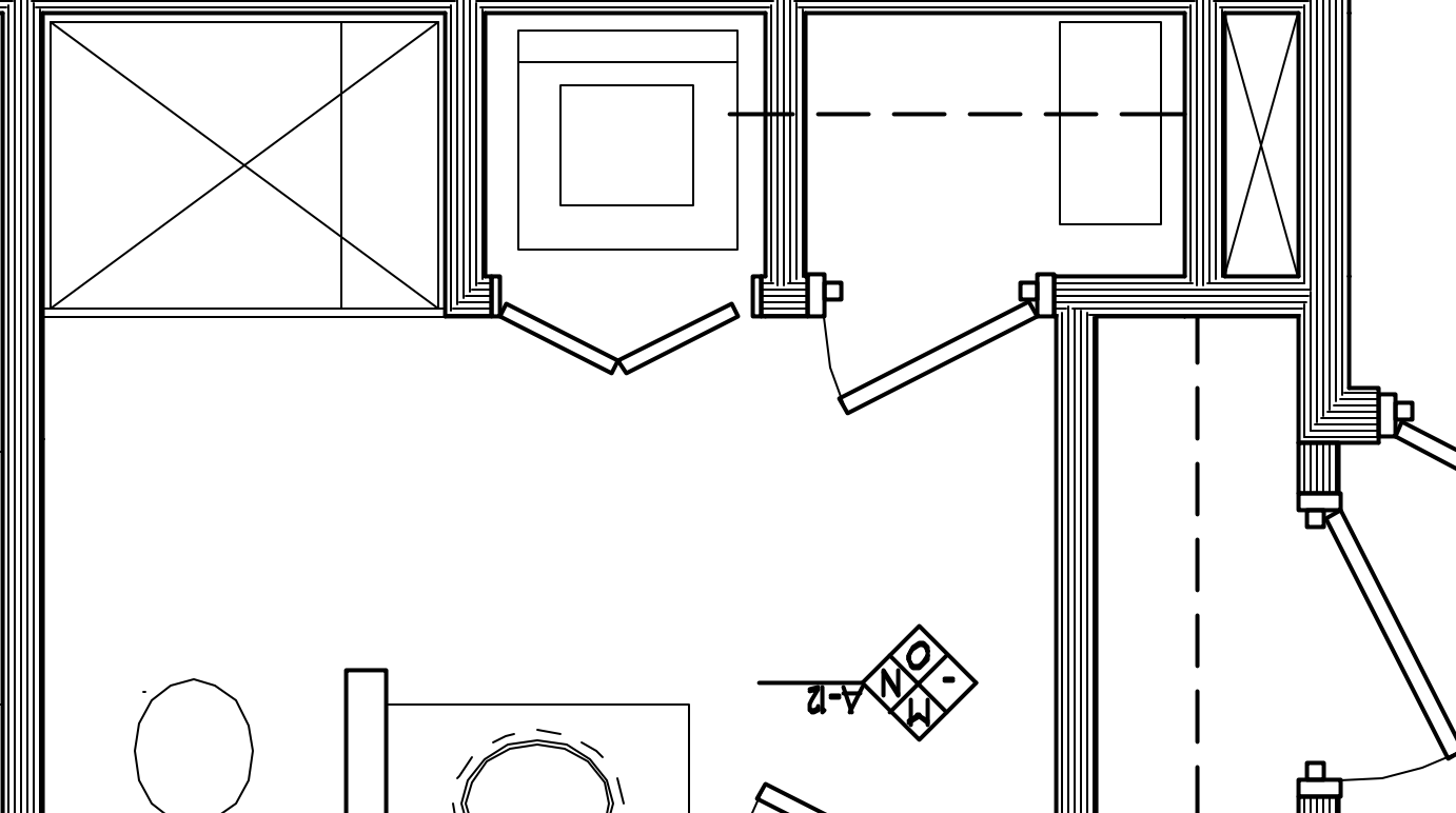
4 ENLARGED BATH PLAN SCALE: 1/2" = 1'-0"
