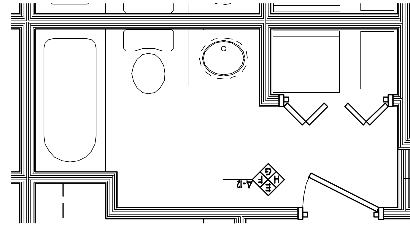
2 ENLARGED BATH PLAN SCALE: 1/2" = 1'-0"
