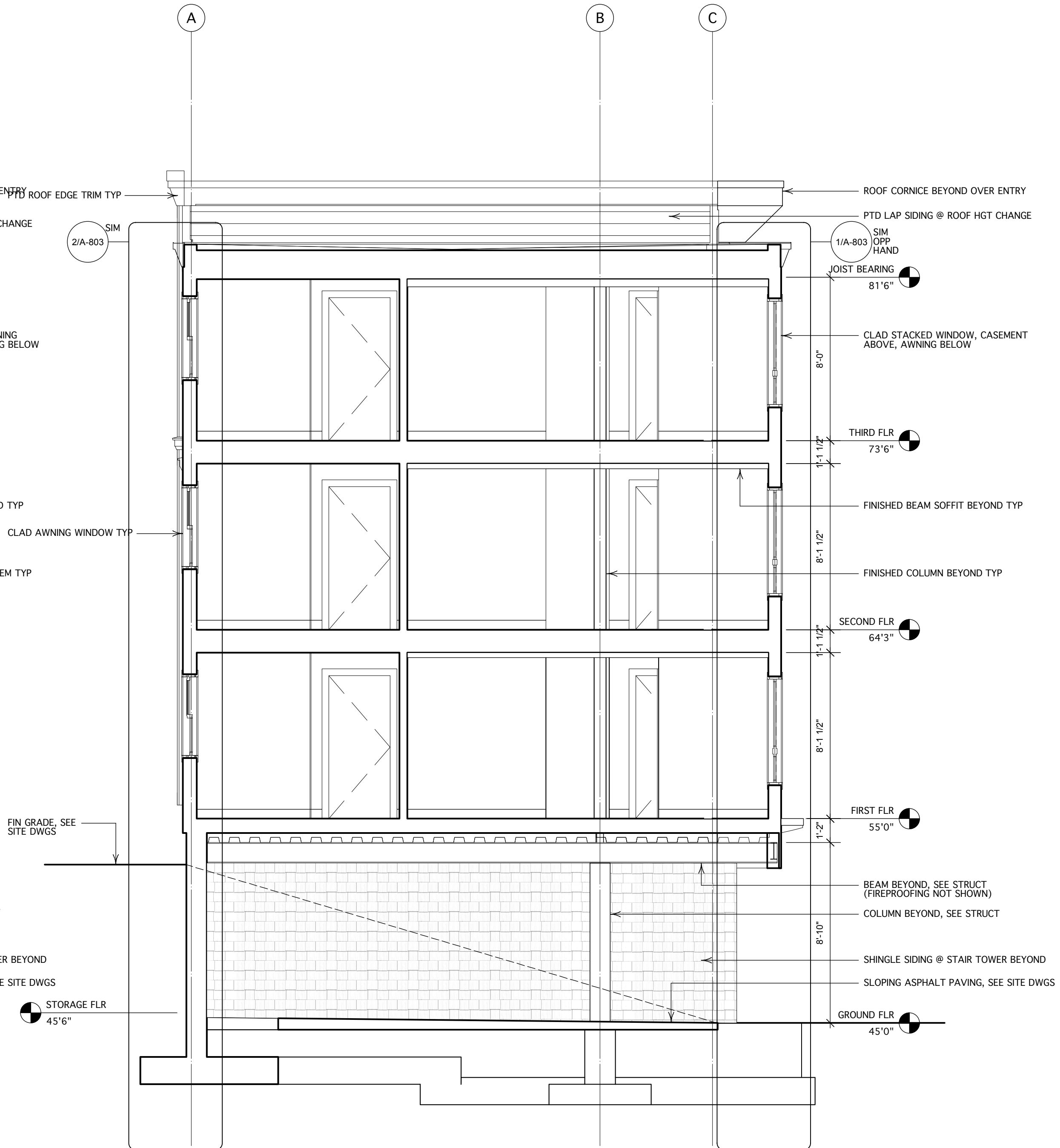
1 BUILDING SECTION - VIEW EAST A-301 Scale: 1/4" = 1'-0"
