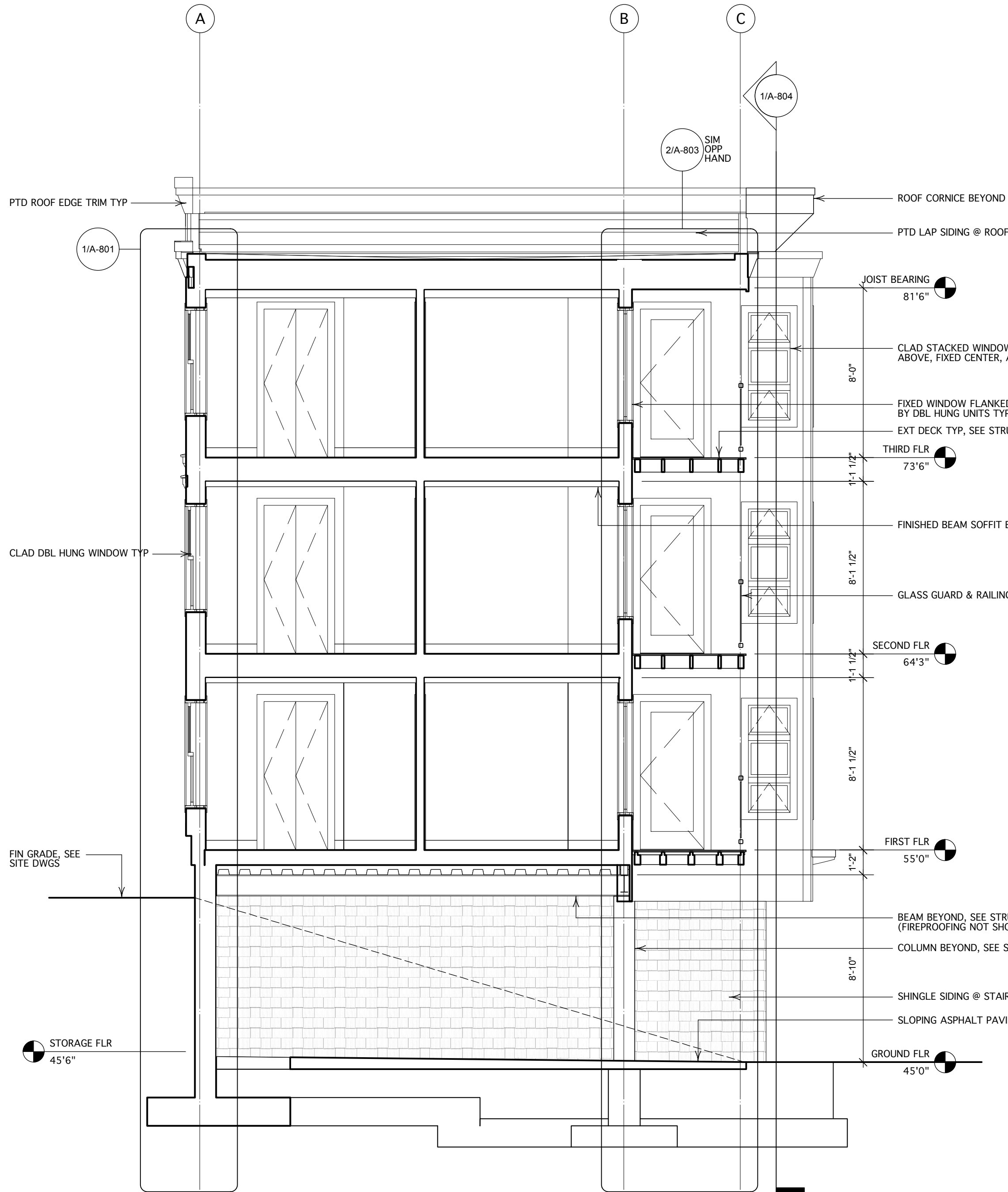
2 BUILDING SECTION - VIEW EAST A-301 Scale: 1/4" = 1'-0"
