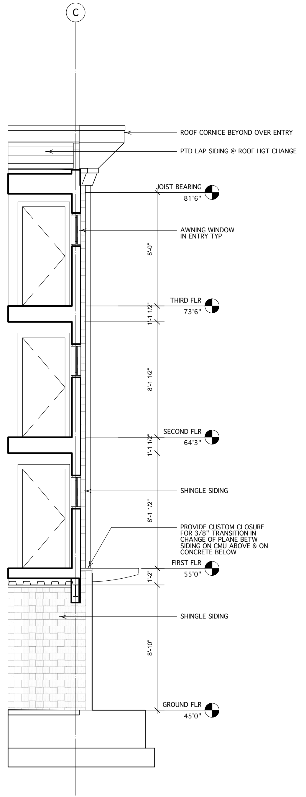
3 PARTIAL SECTION - VIEW SHINGLE SIDING ON STAIR A-301 Scale: 1/4" = 1'-0"
