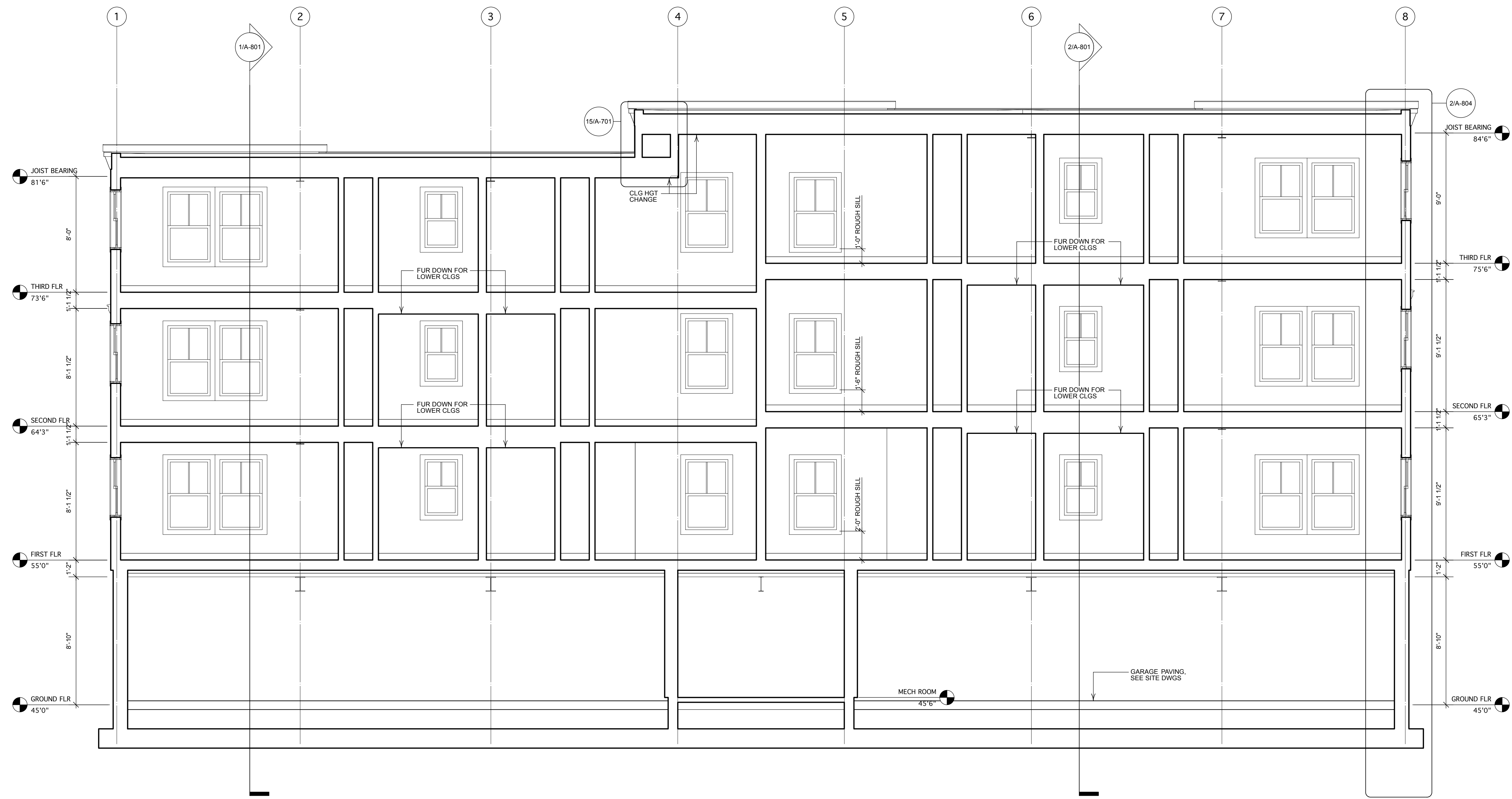
1 BUILDING SECTION VIEW NORTH Scale: 1/4" = 1'-0"
