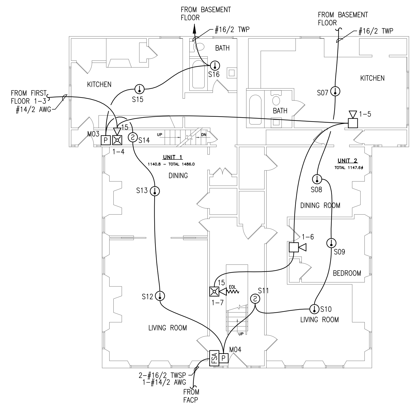
FIRST FLOOR FIRE ALARM PLAN SCALE: 1/8"=1'-0" 0 4' 8' 16'
