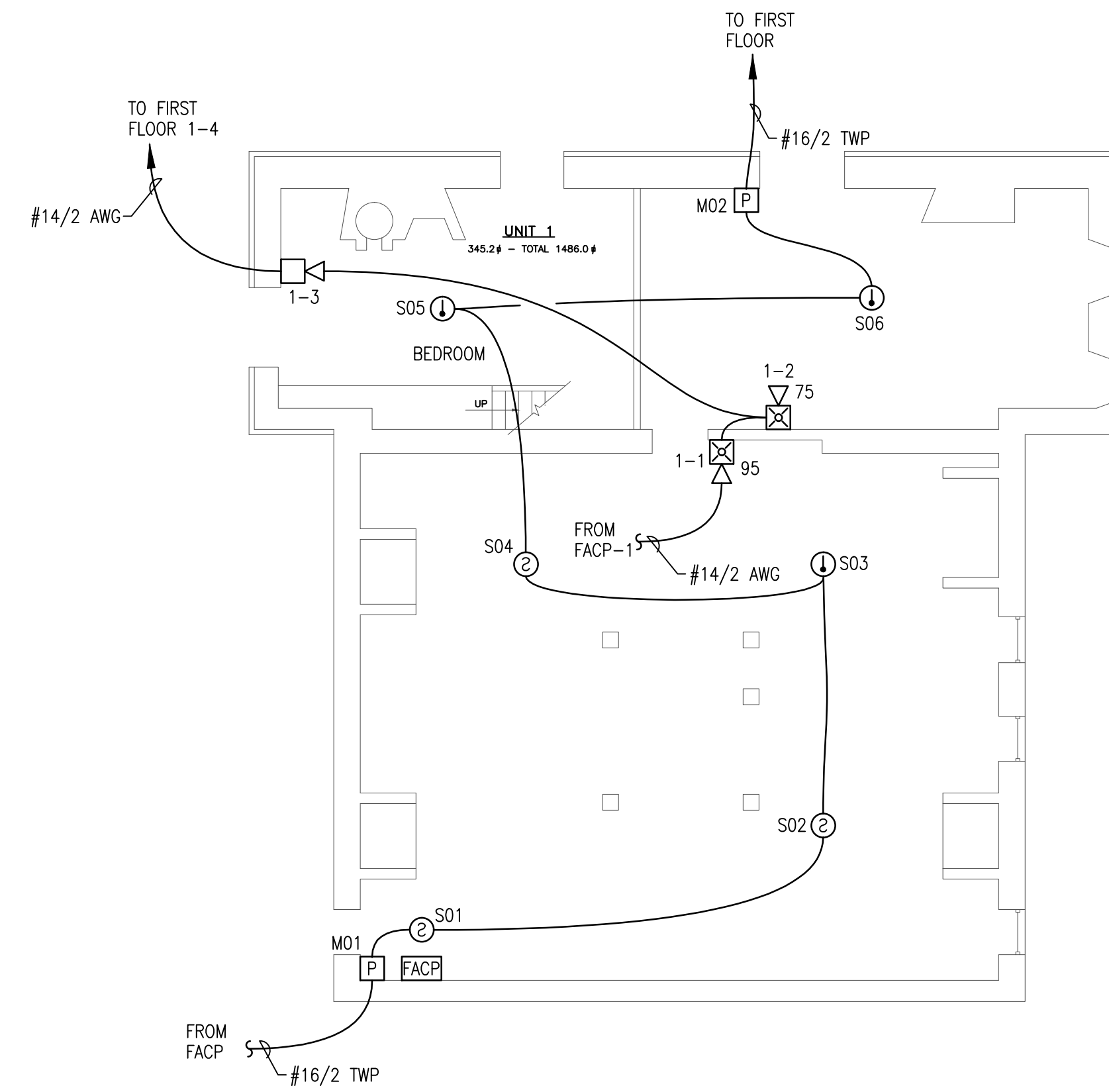
BASEMENT FLOOR FIRE ALARM PLAN SCALE: 1/8"=1'-0"
