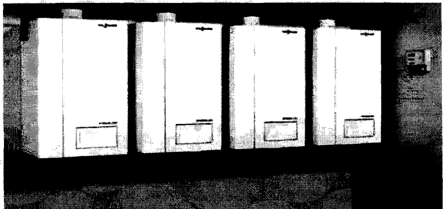
Multi-Vitodens 200 installation
