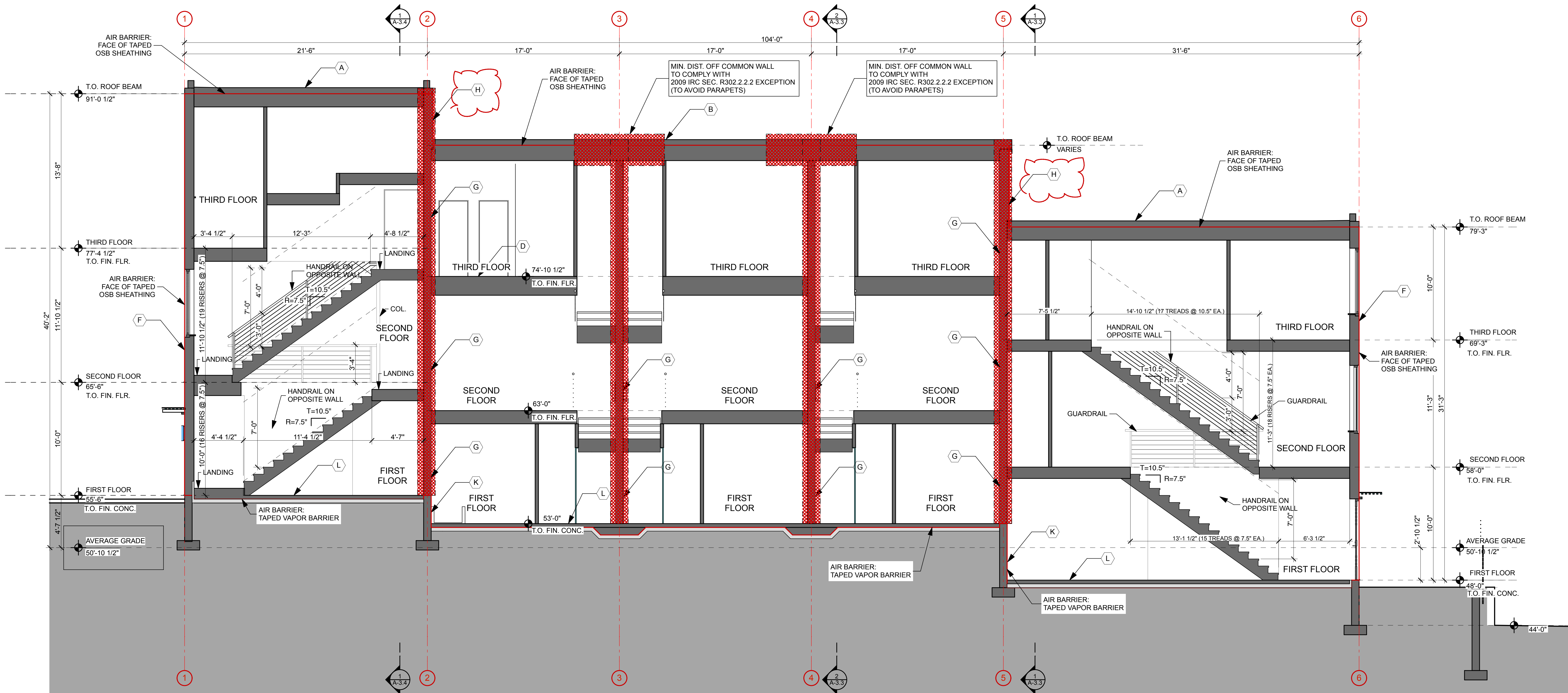
1 SECTION: LENGTH STAIRS SCALE: 1/4" = 1'-0"
