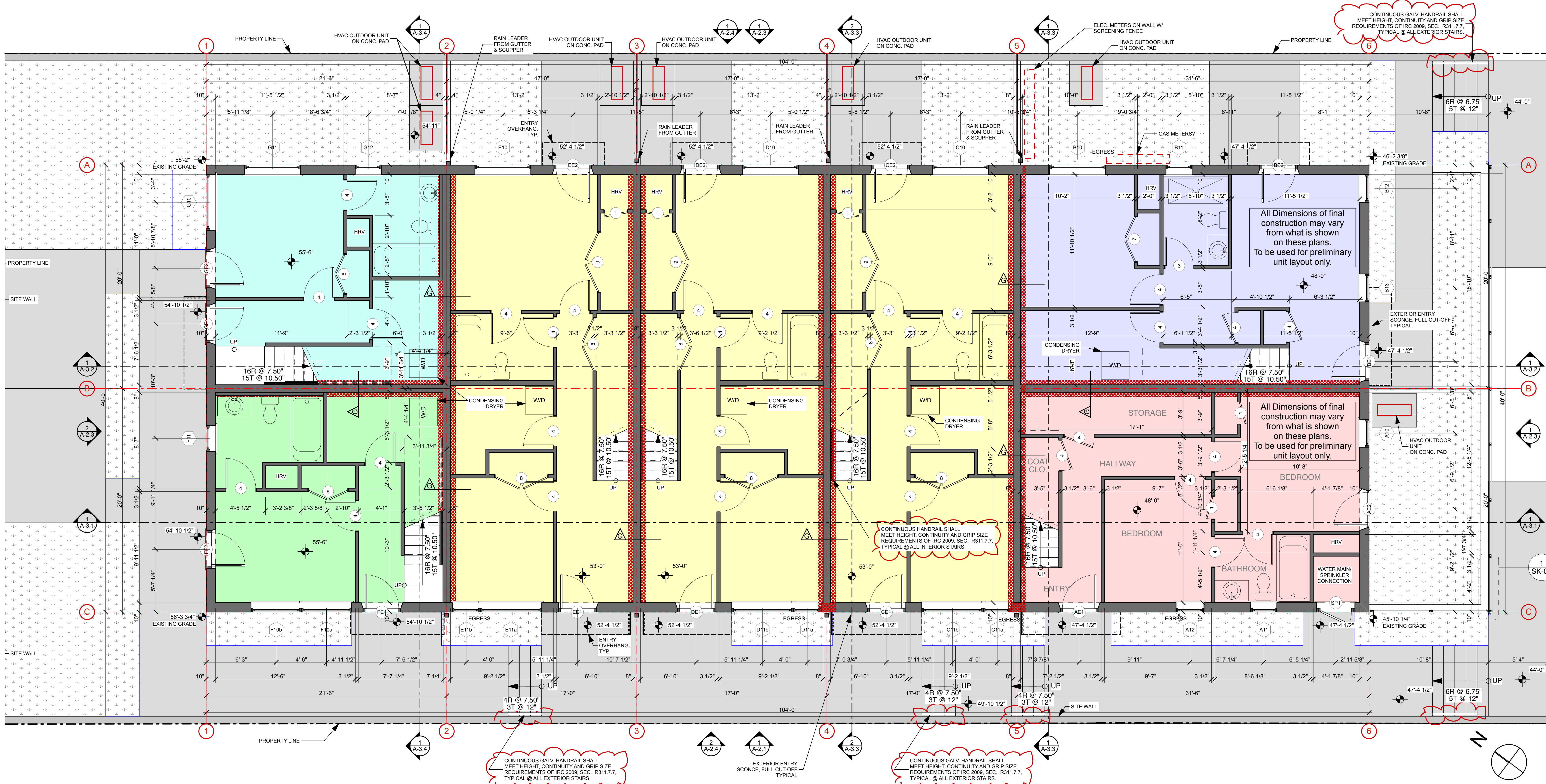
1 1st FLOOR SCALE: 1/4" = 1'-0"
