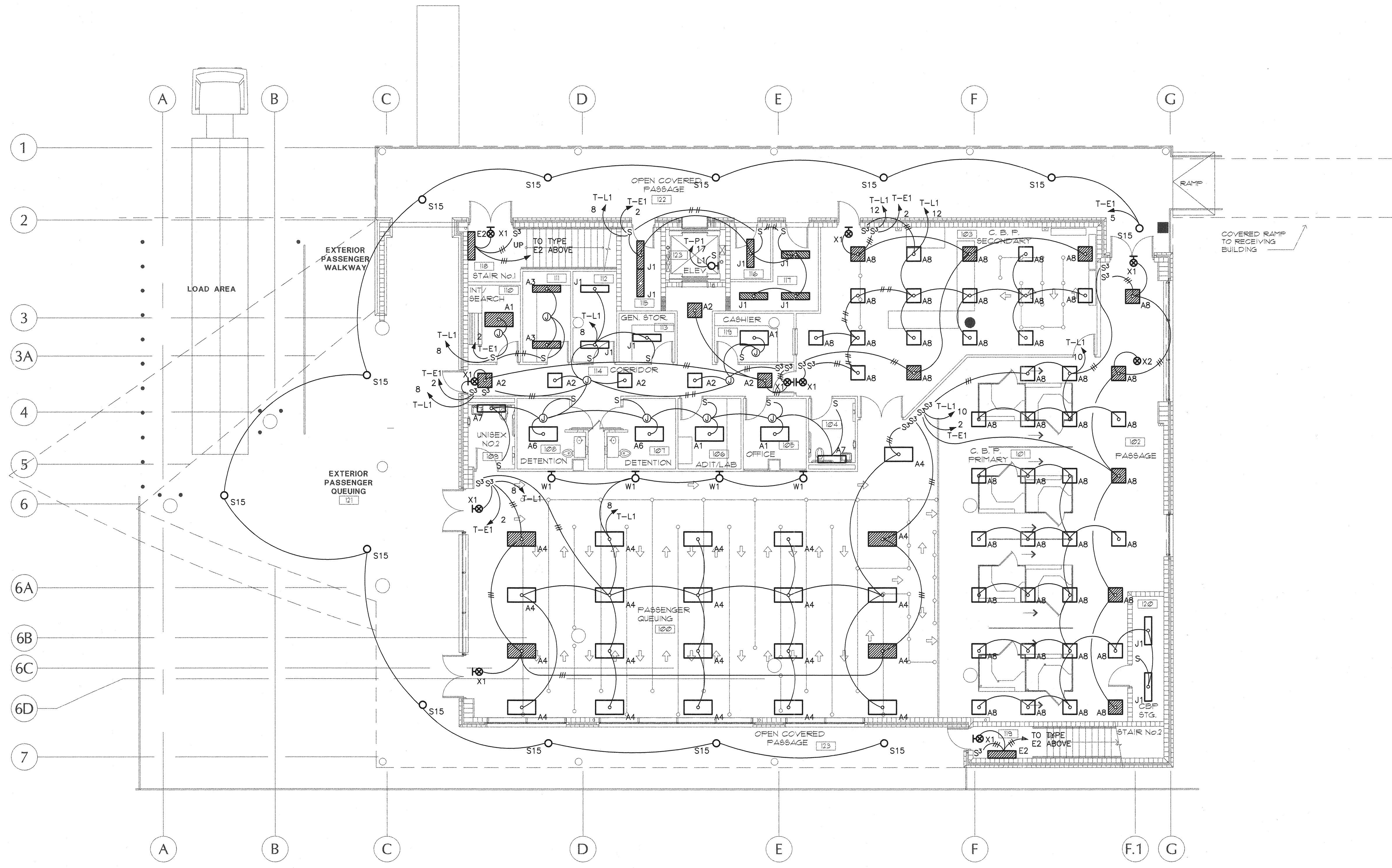
1 FIRST FLOOR LIGHTING PLAN 1/8" = 1'-0"
