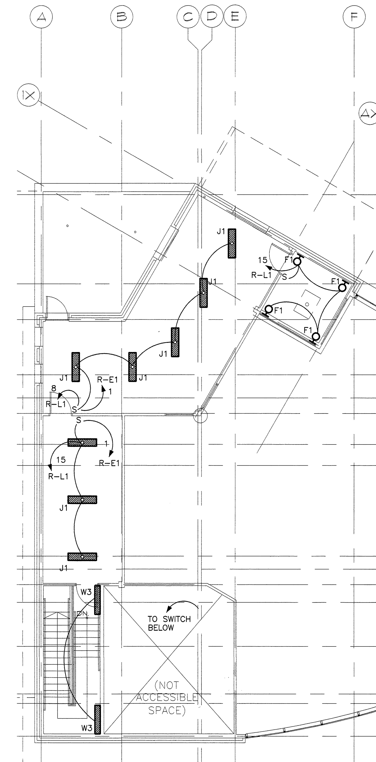
2 MEZZANINE LIGHTING PLAN 1/8" = 1'-0"
