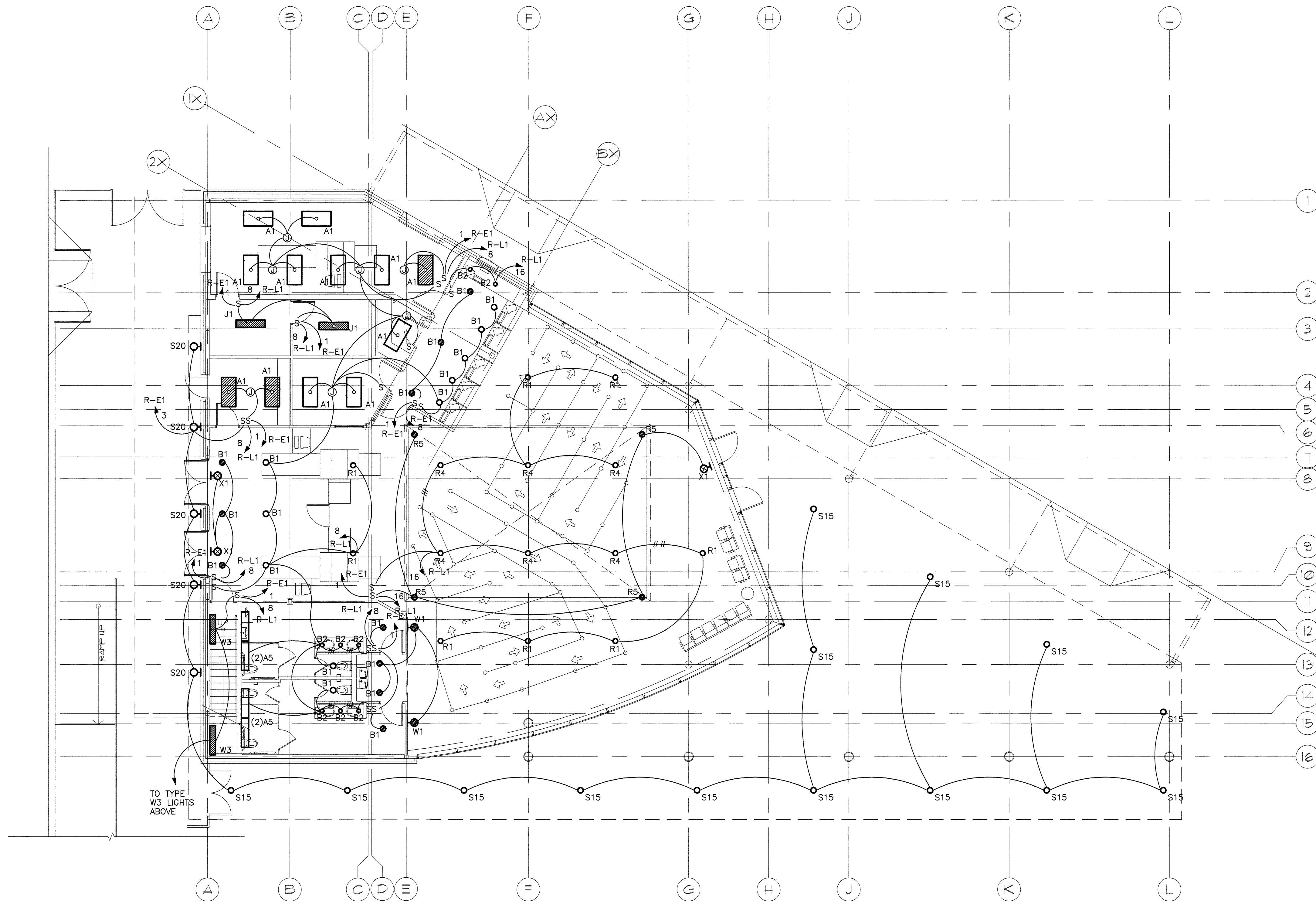
1 MAIN FLOOR LIGHTING PLAN 1/8" = 1'-0"
