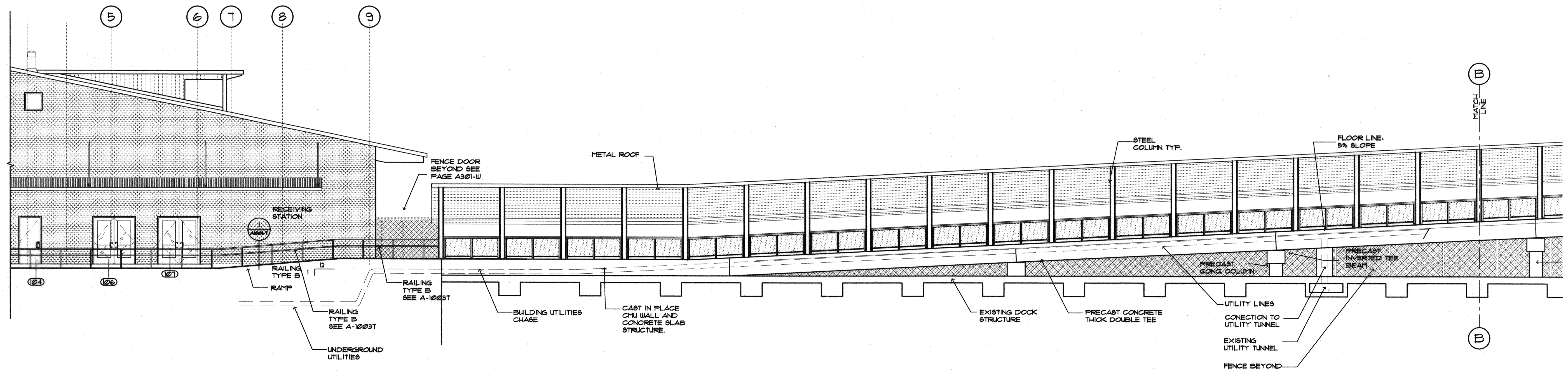
WEST PARTIAL ELEVATION SCALE 1/8" = 1'-0"
