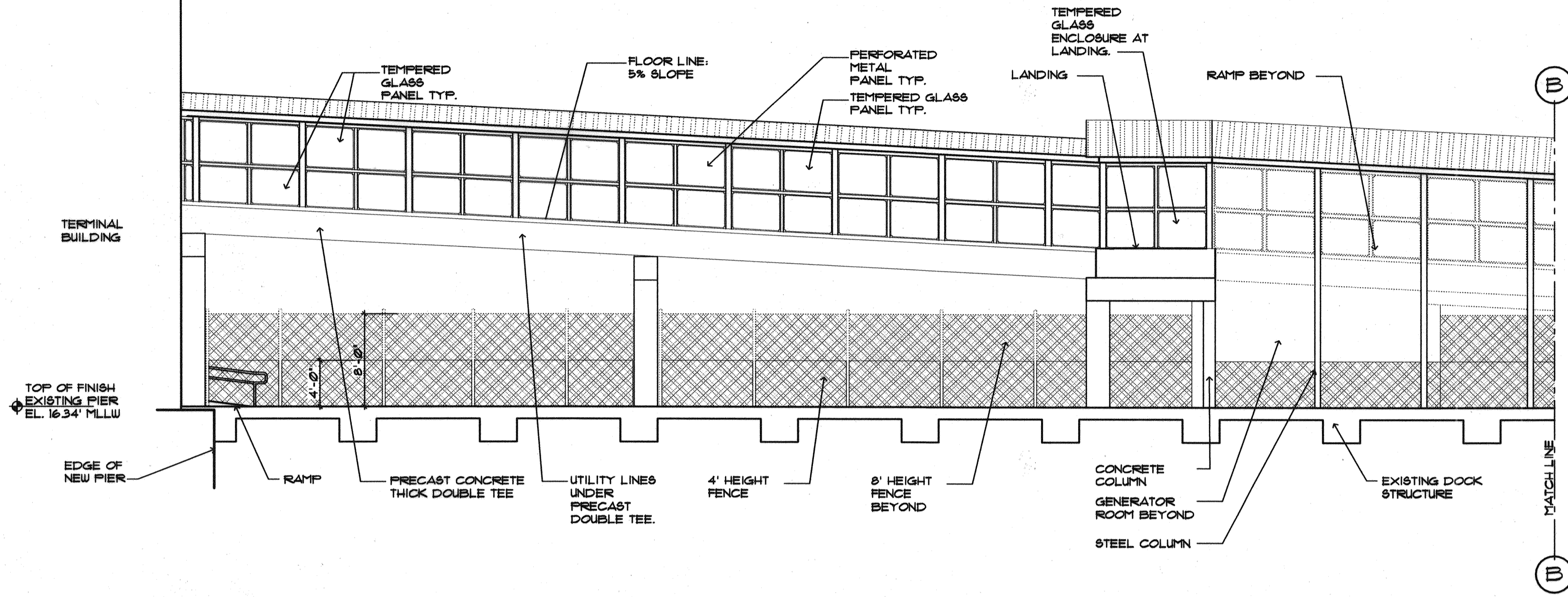
EAST PARTIAL ELEVATION SCALE 1/8" = 1'-0"
