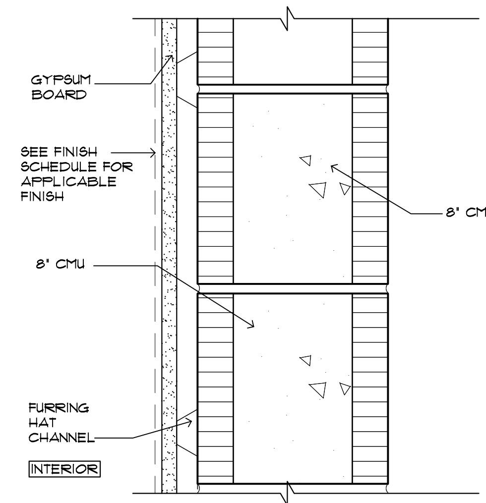
M-3 M-3A 2 HR. FIRE RATING UL-U905
