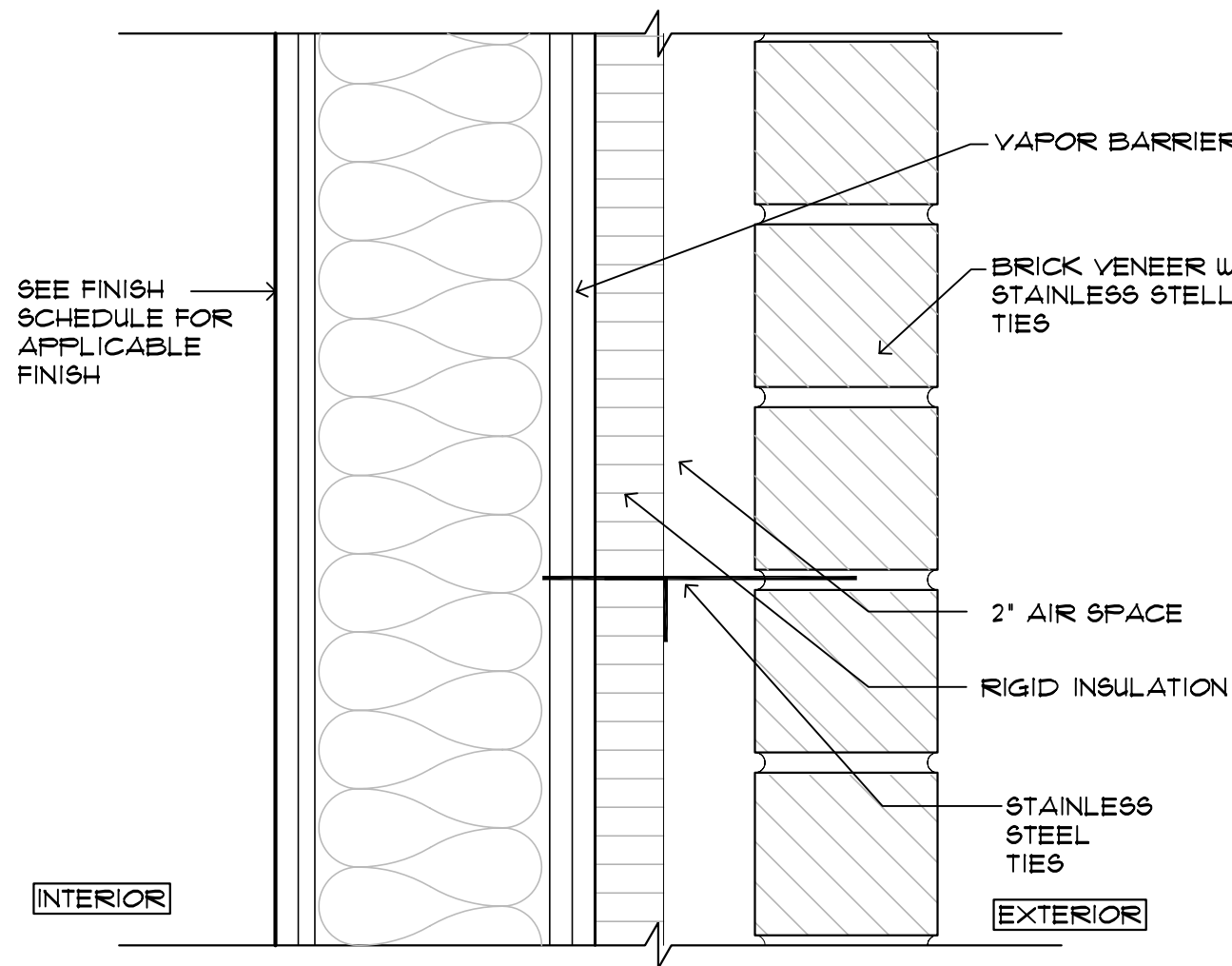
M-1 R=20 TYPICAL M-1A 2 HR. FIRE RATING UL-U419
