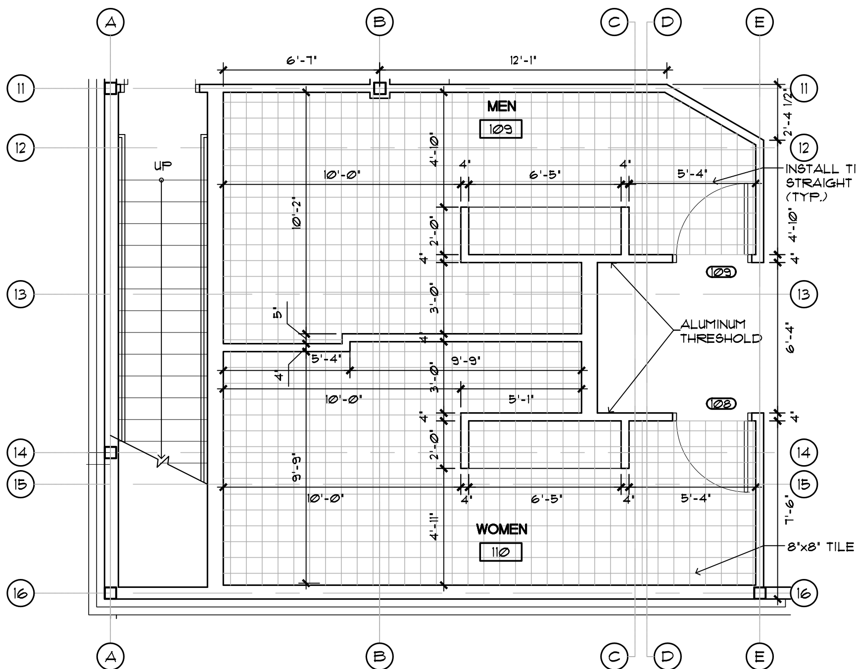
ENLARGED RESTROOM FLOOR TILE PLAN SCALE: 1/4"=1'-0"
