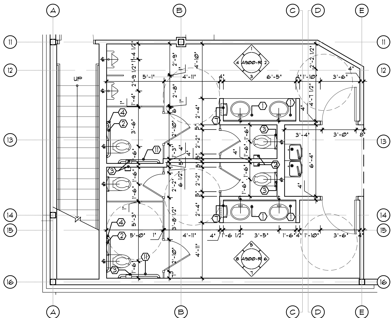
ENLARGED RESTROOM FLOOR PLAN SCALE: 1/4"=1'-0"
