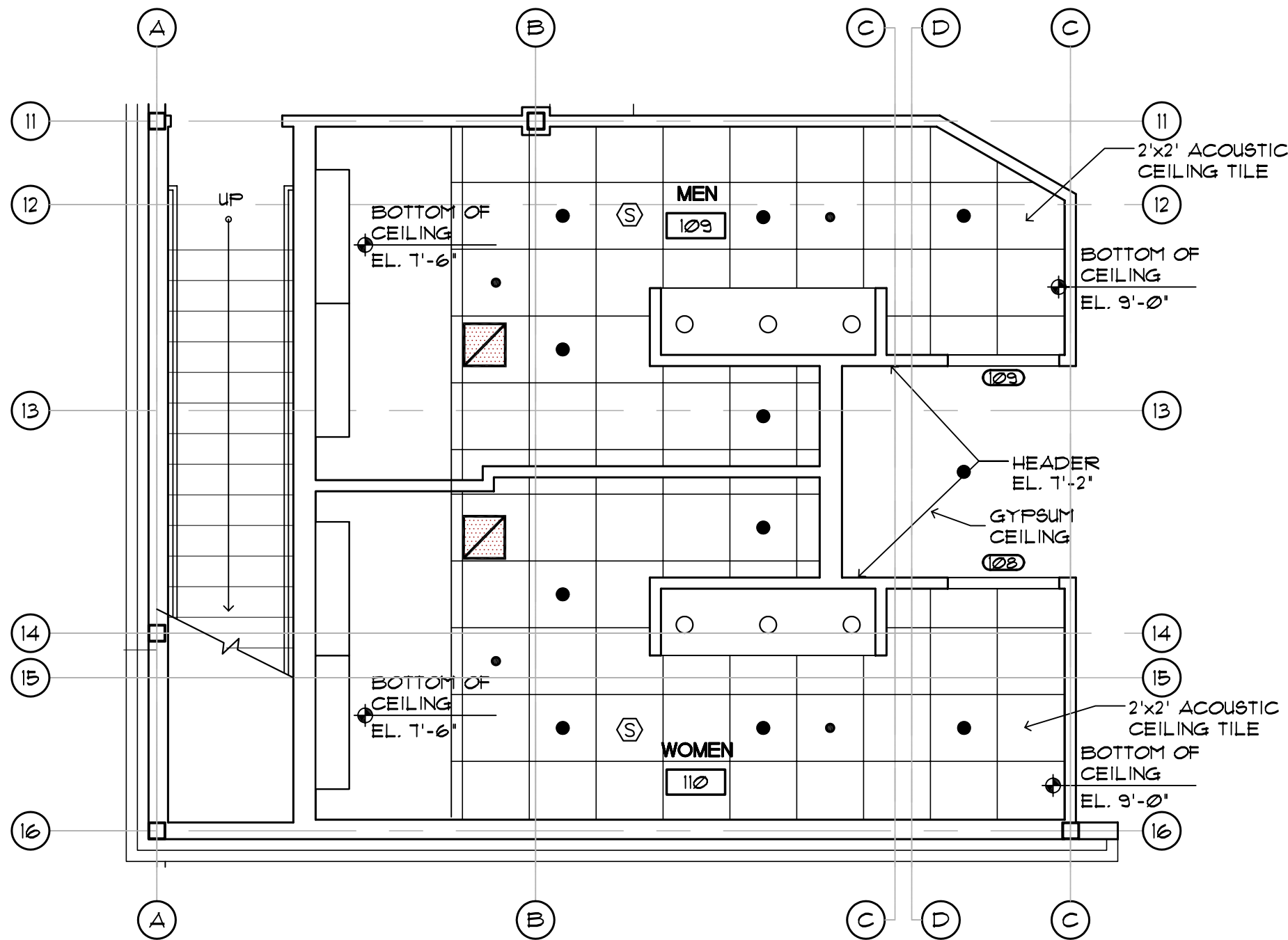
ENLARGED RESTROOM REFLECTED CEILING PLAN SCALE: 1/4"=1'-0"
