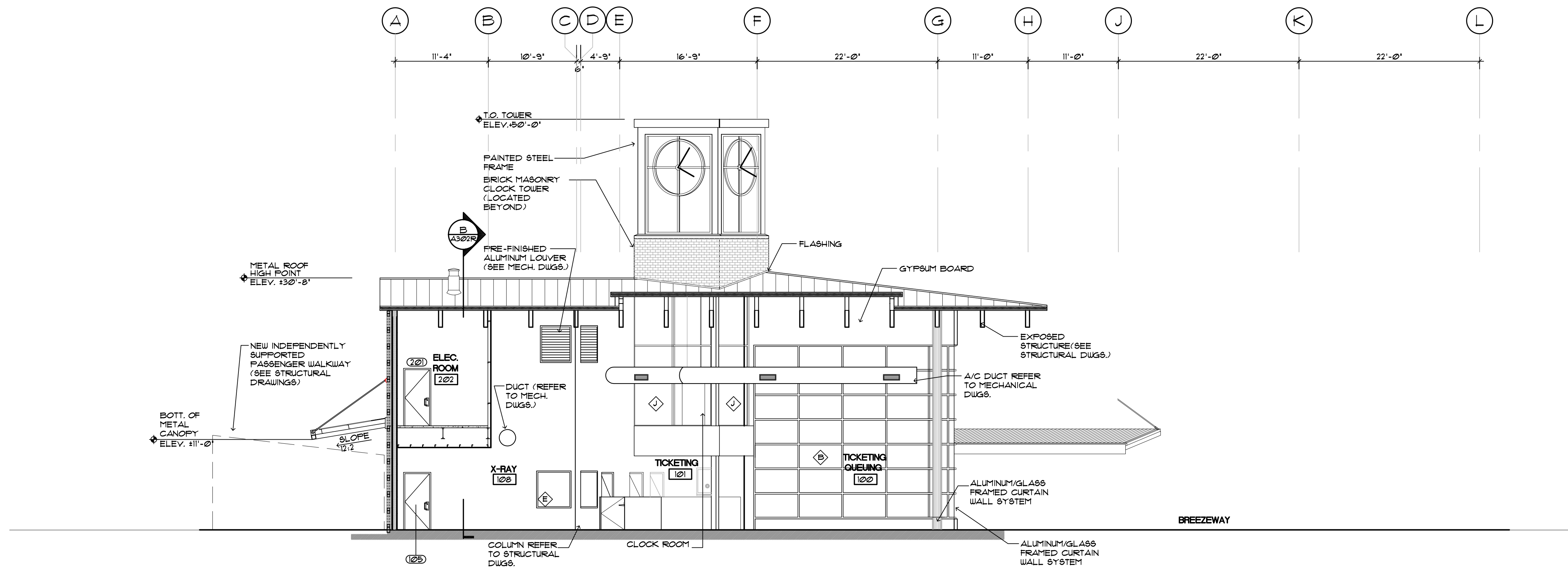
BUILDING SECTION C-C SCALE: 1/8" = 1'-0"
