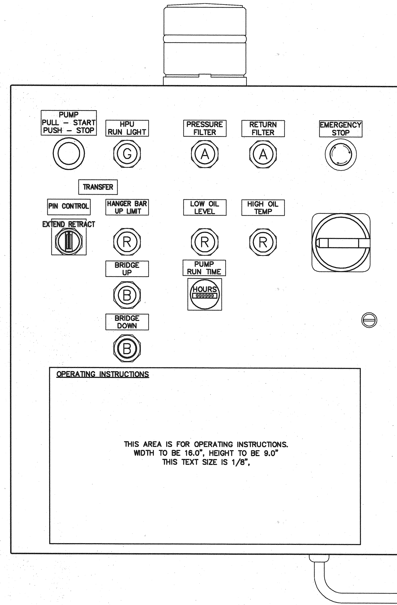
CONTROL PANEL NOT TO SCALE
