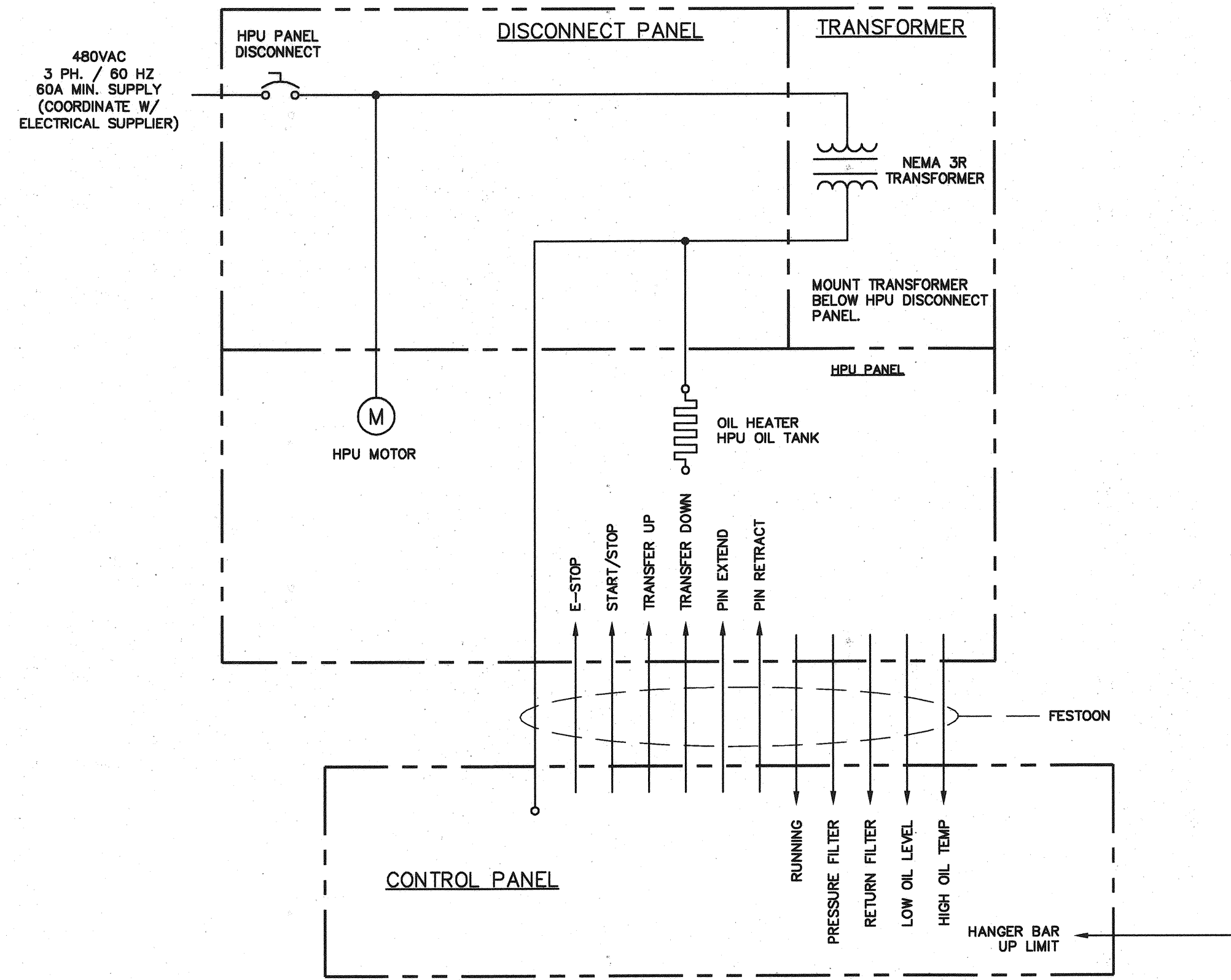
WIRING DIAGRAM NOT TO SCALE
