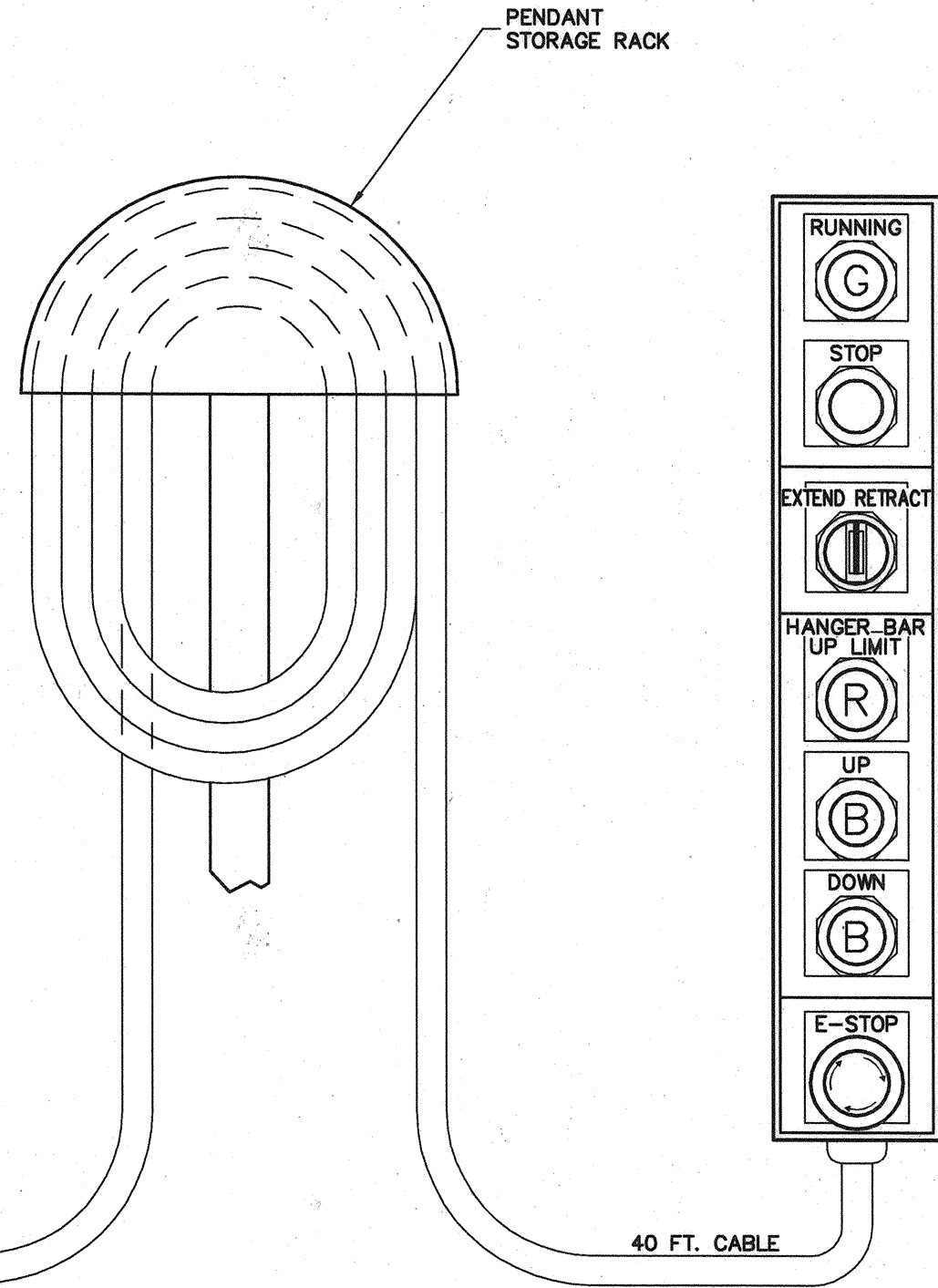
PENDANT NOT TO SCALE
