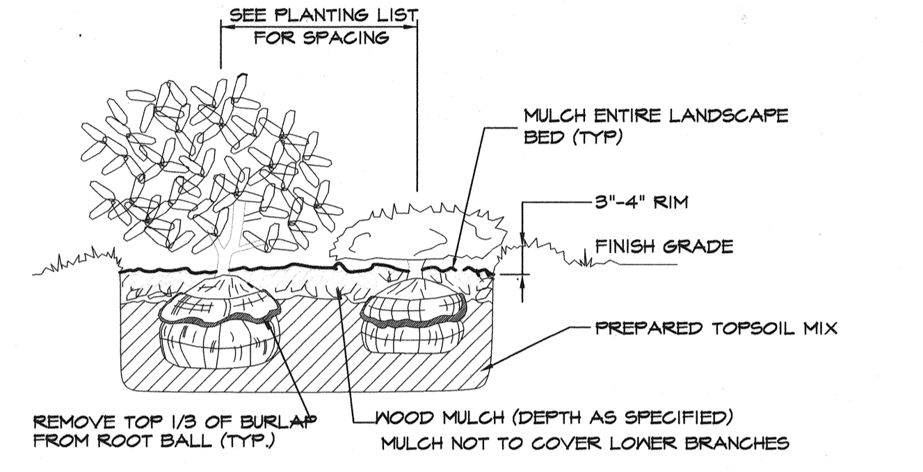
2 SHRUB PLANTING DETAIL NOT TO SCALE
