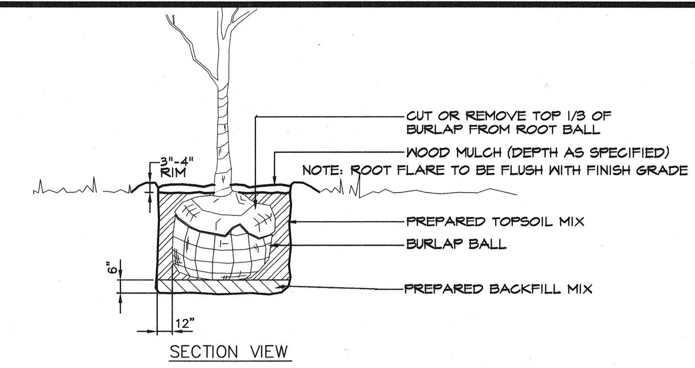
1 TREE PLANTING DETAIL NOT TO SCALE
