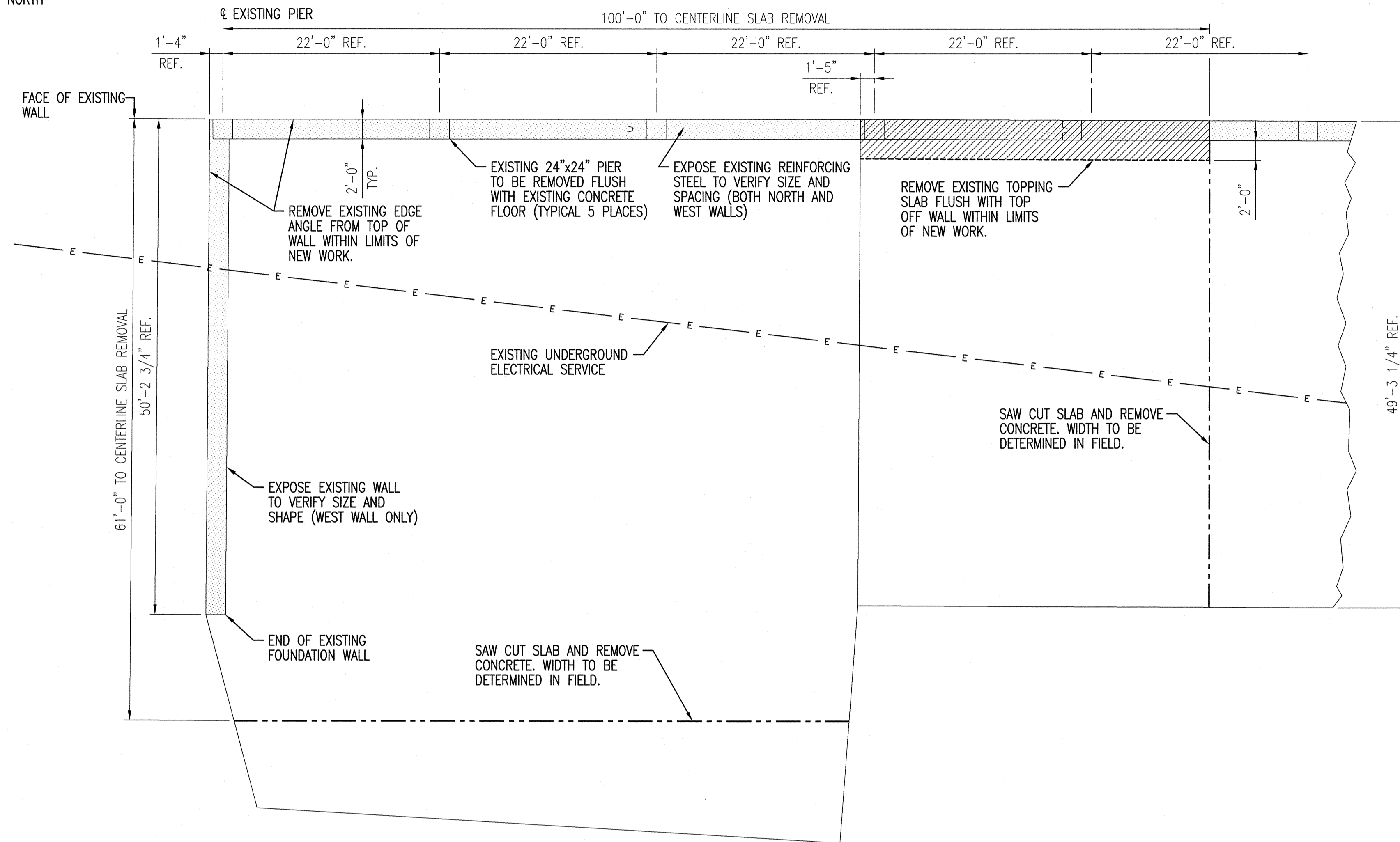
DEMOLITION PLAN SCALE: 1/8"=1'-0"
