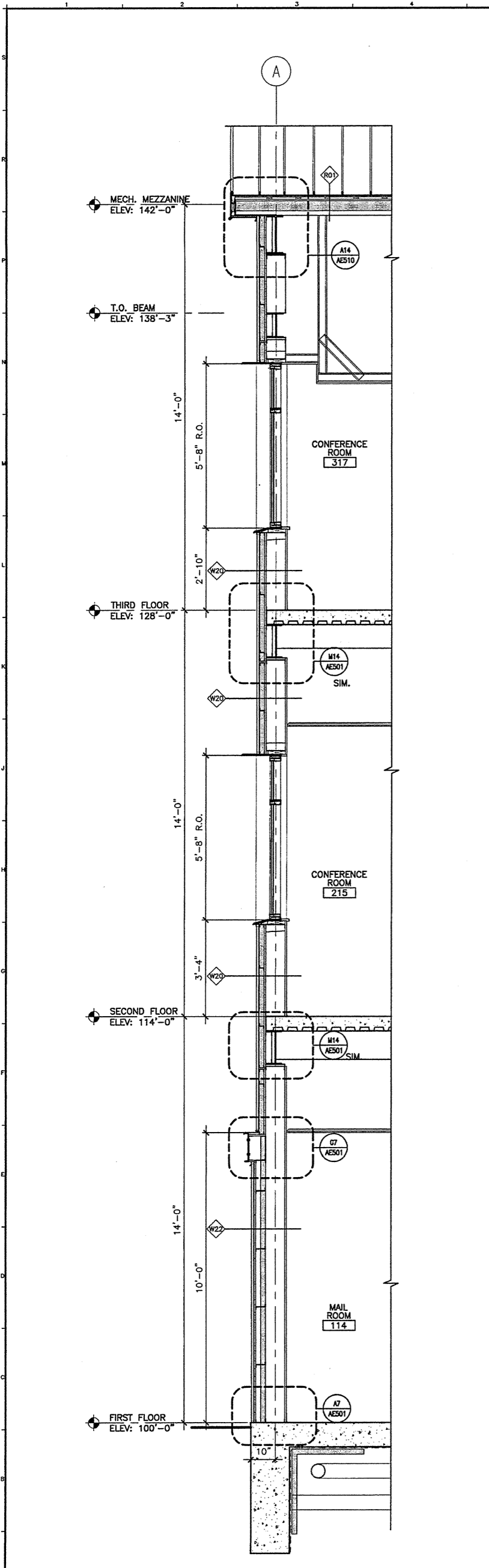
A1 WALL SECTION 1/2" = 1'-0" AE101, AE102, AE103, AE104, AE202
