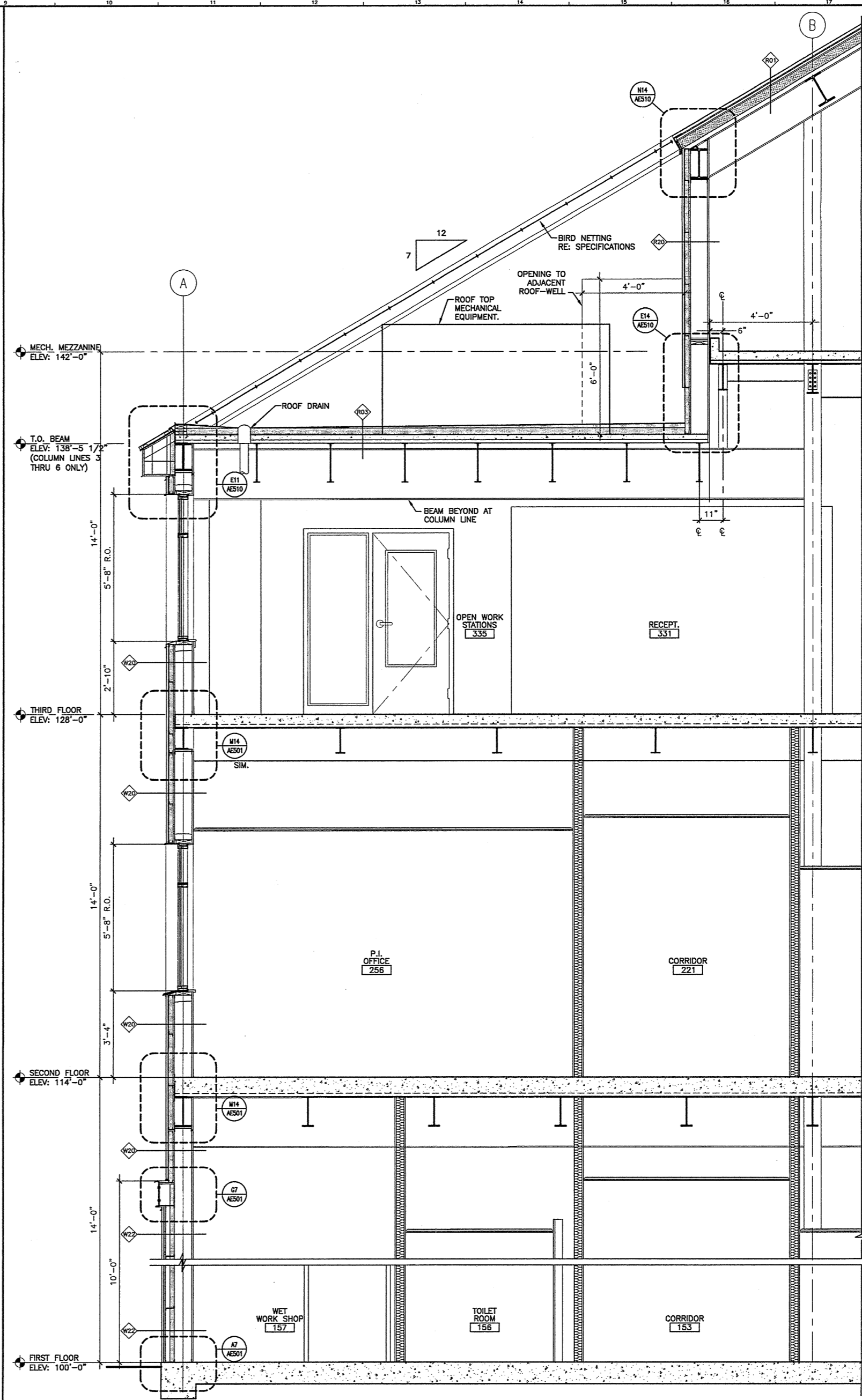
A9 WALL SECTION 1/2" = 1'-0" AE101, AE102, AE103, AE104, AE202, AE302
