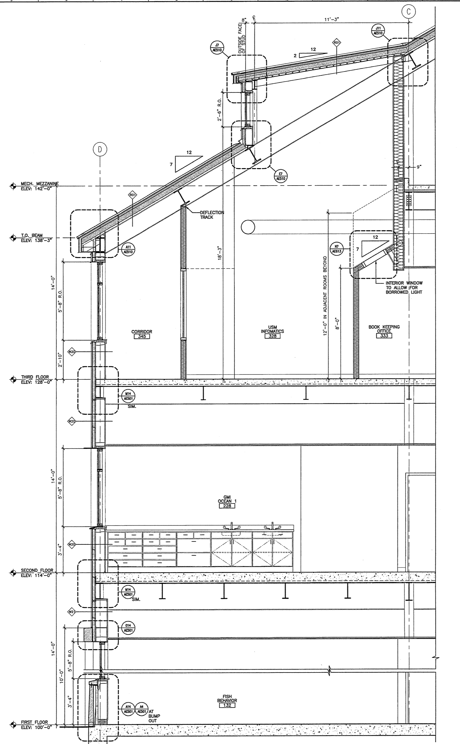
A5 WALL SECTION 1/2" = 1'-0" AE101, AE102, AE103, AE104, AE201, AE302
