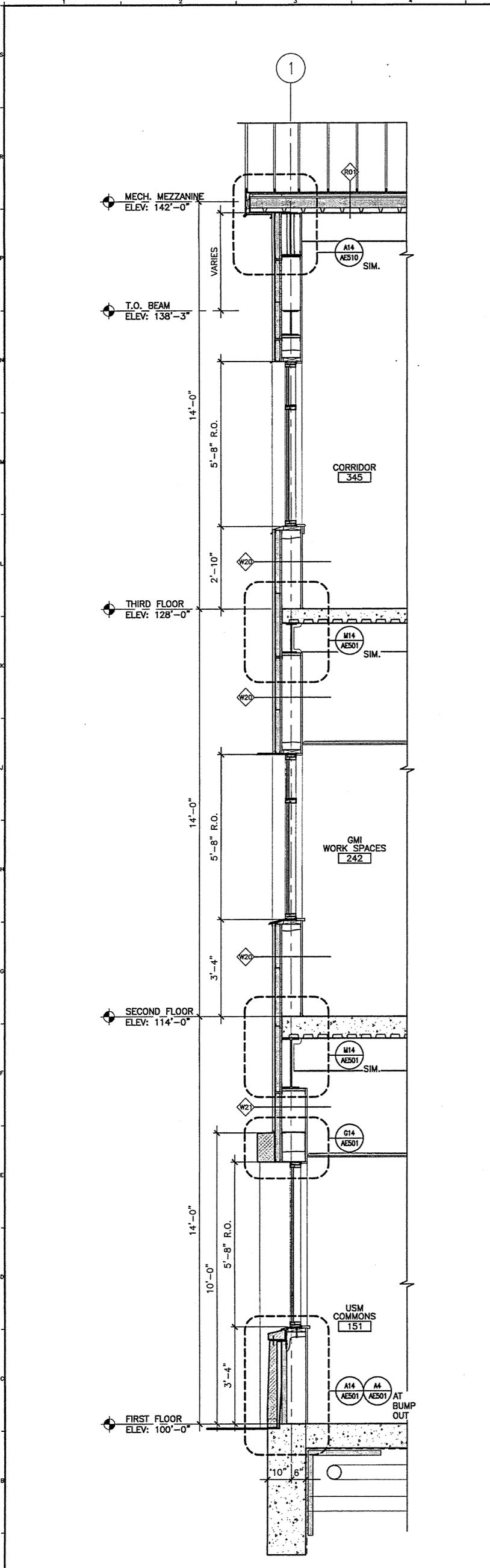
A1 WALL SECTION 1/2" = 1'-0" AE101, AE102, AE103, AE104, AE202, AE301
