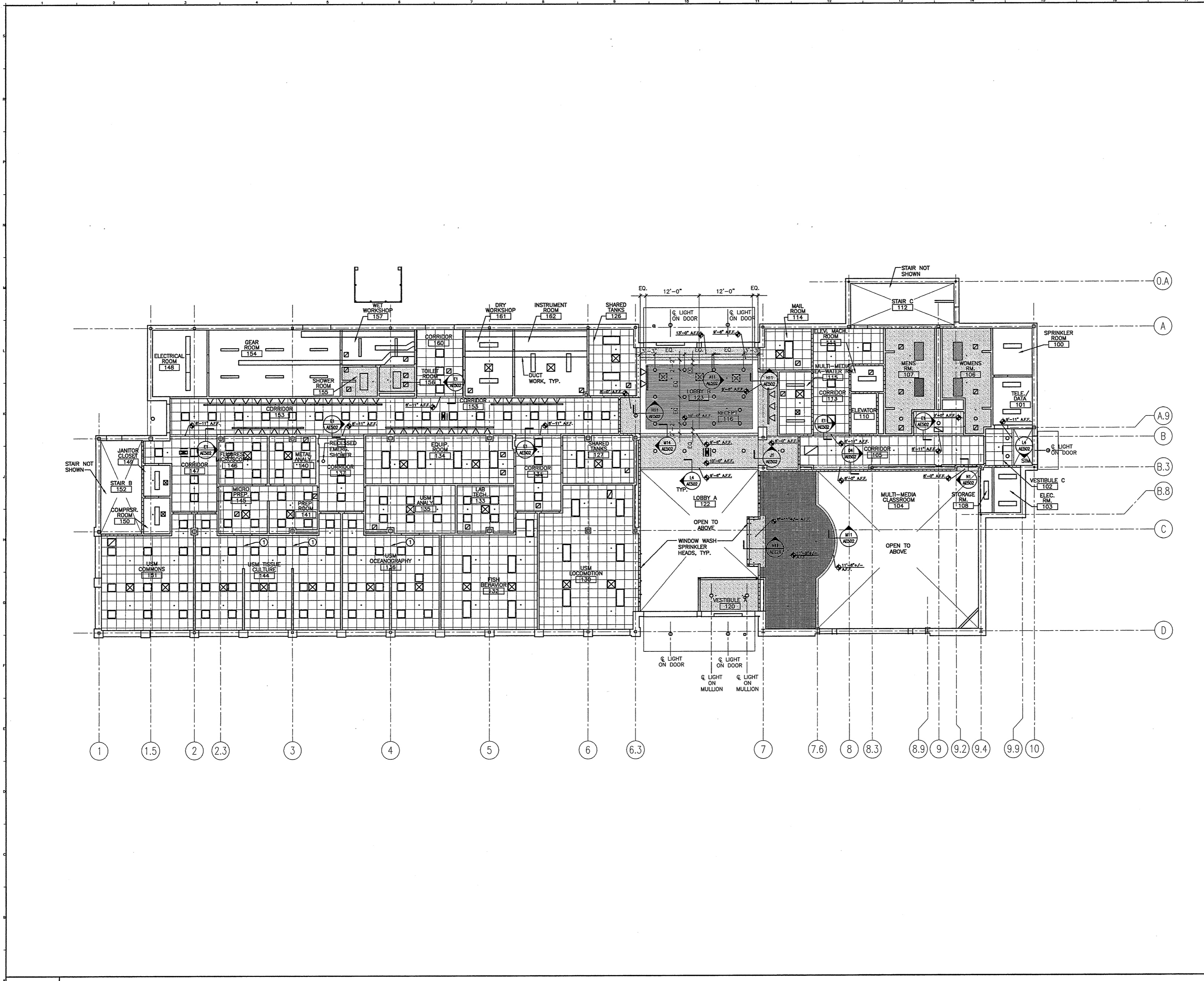
A1 FIRST FLOOR REFLECTED CEILING PLAN
