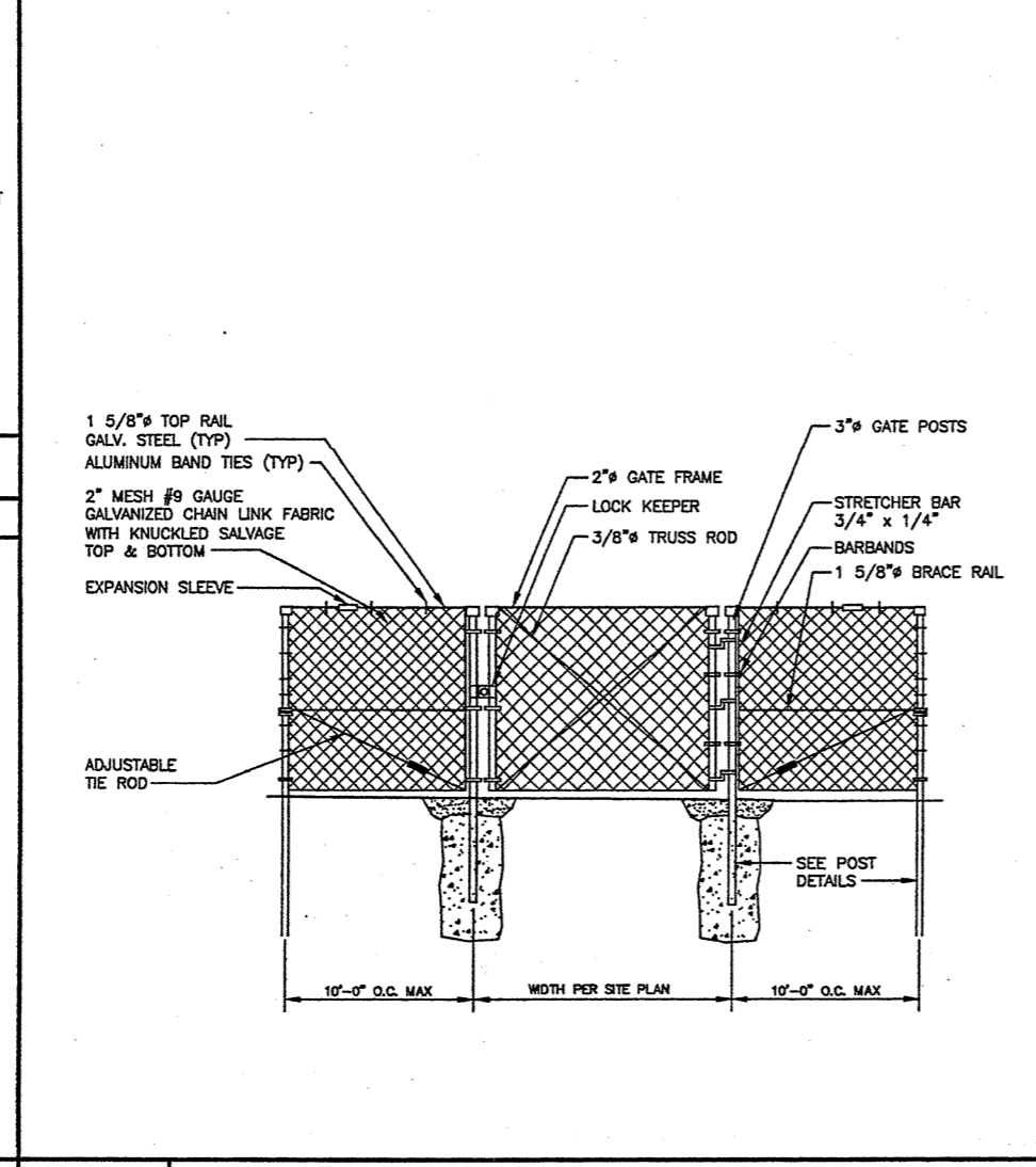
A5 SINGLE LEAF GATE DETAIL N.T.S.
