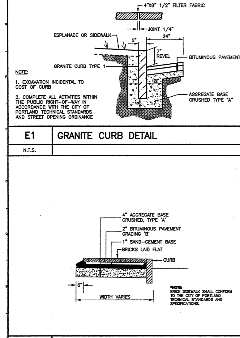
A1 BRICK WITH BITUMINOUS BASE SIDEWALK N.T.S.
