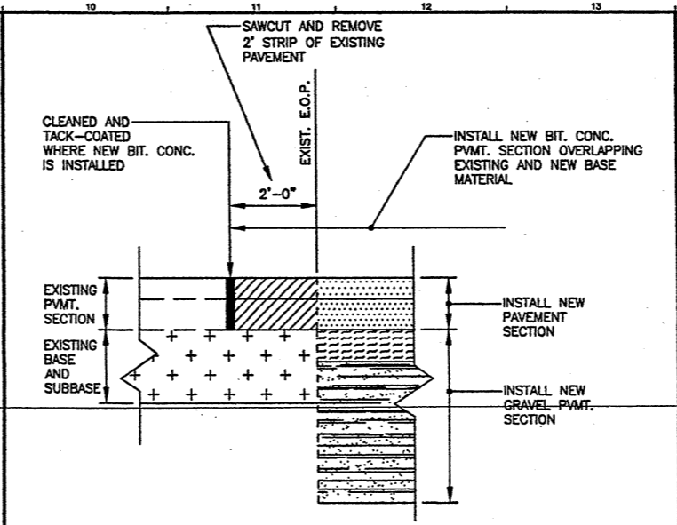
H1 TYPICAL UNDERDRAIN TRENCH SECTION N.T.S.
