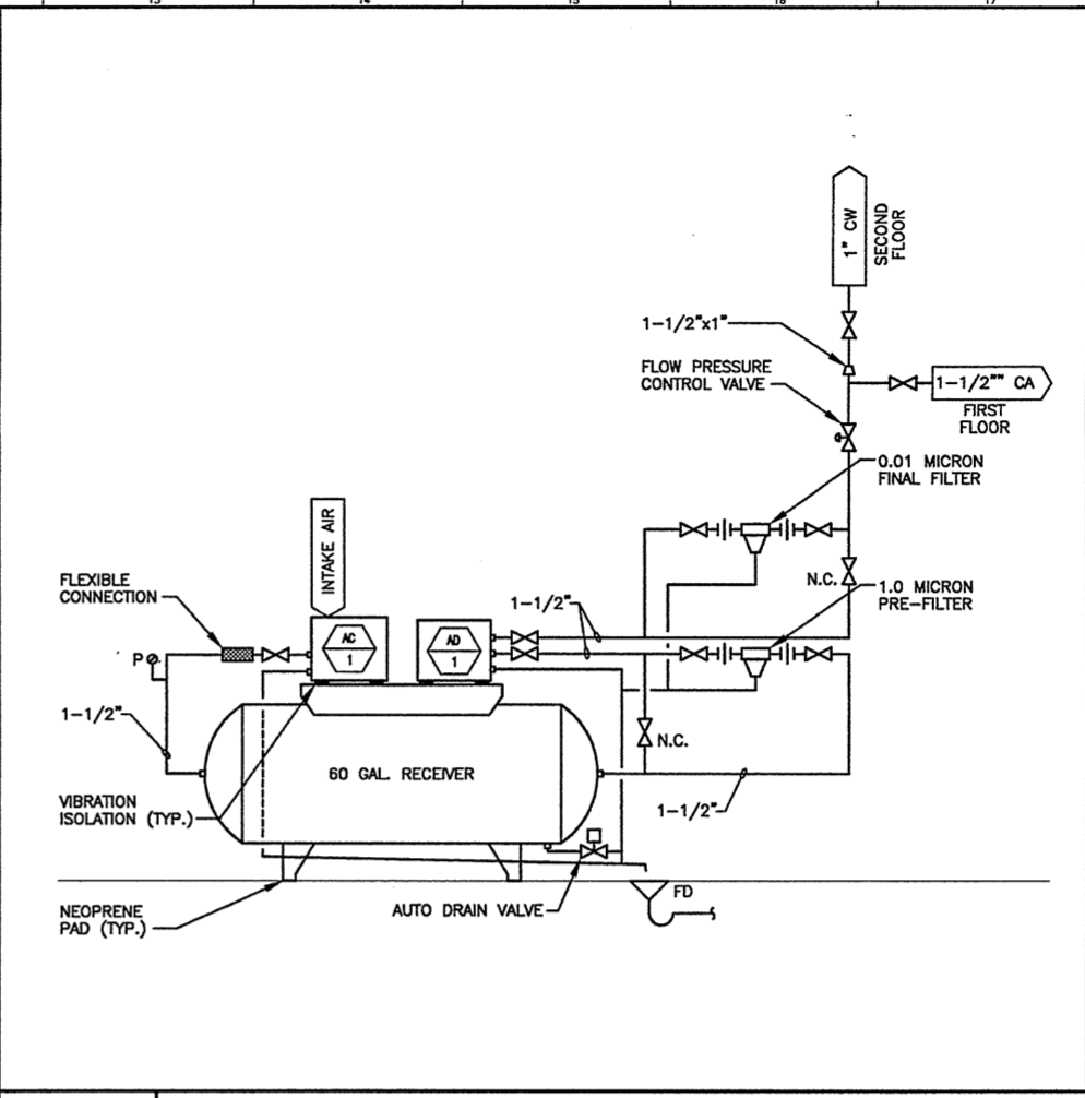
L13 COMPRESSED AIR SCHEMATIC NOT TO SCALE
