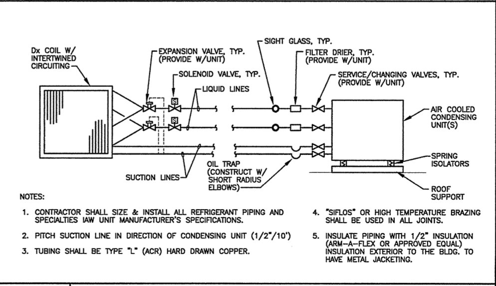
A13 REFRIGERANT PIPING SCHEMATIC NOT TO SCALE
