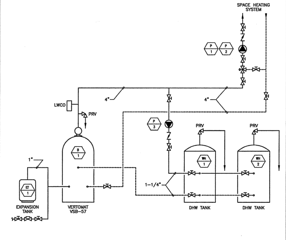
E13 PIPING DIAGRAM NOT TO SCALE
