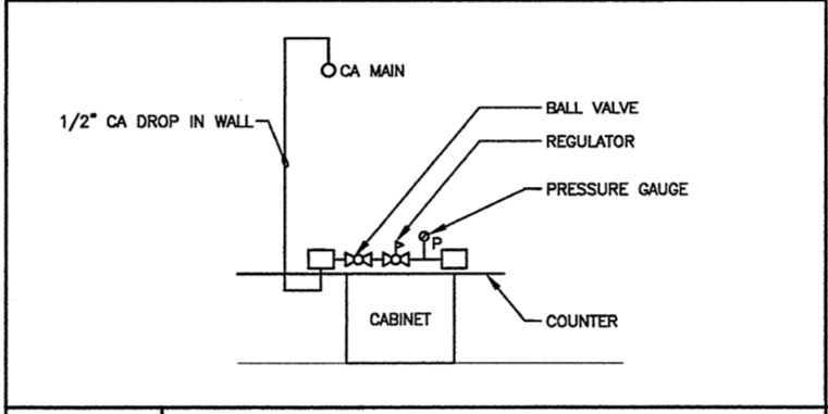
L9 LAB BENCH CA (TYP.) NOT TO SCALE
