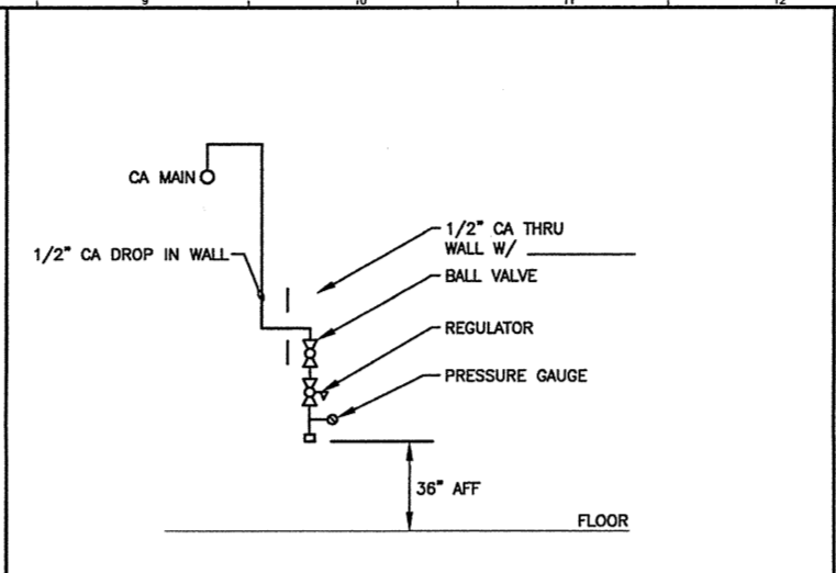
N9 CA DROP (TYP.) NOT TO SCALE
