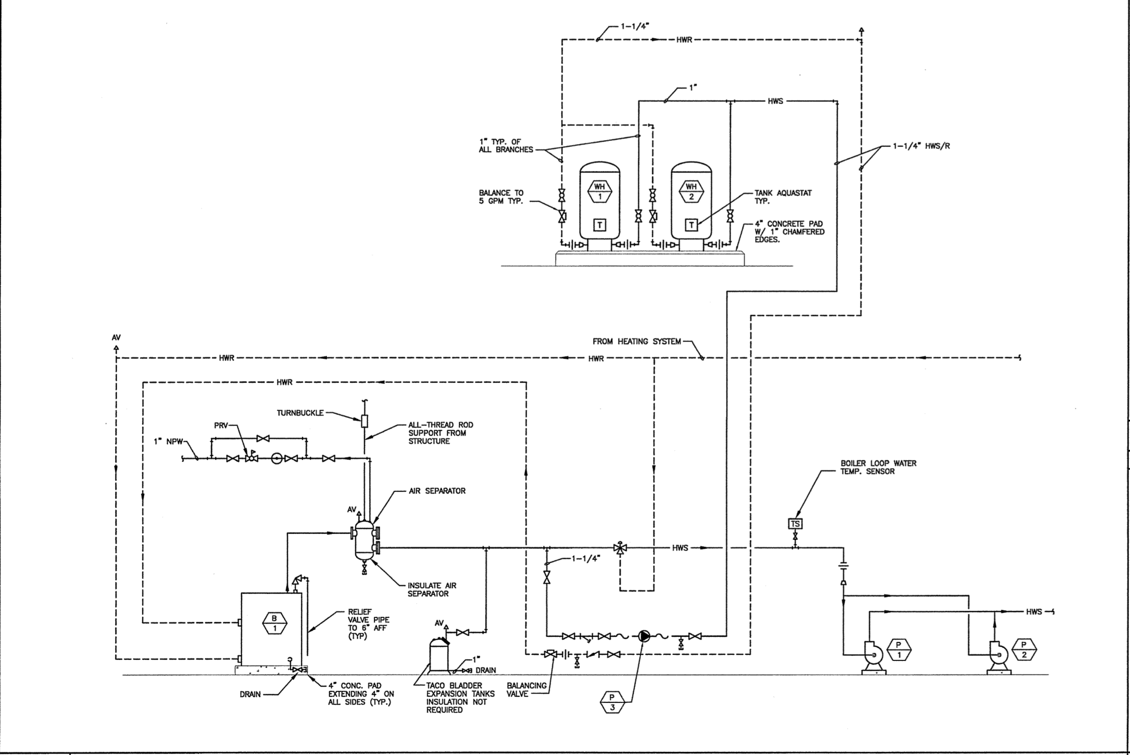
A1 HYDRONIC HEATING/DHW SYSTEM SCHEMATIC NOT TO SCALE
