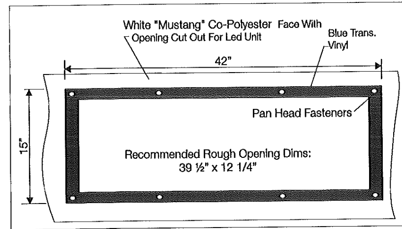
B LED Price Changer Attachment Details Scale: 1"=1'-0"
