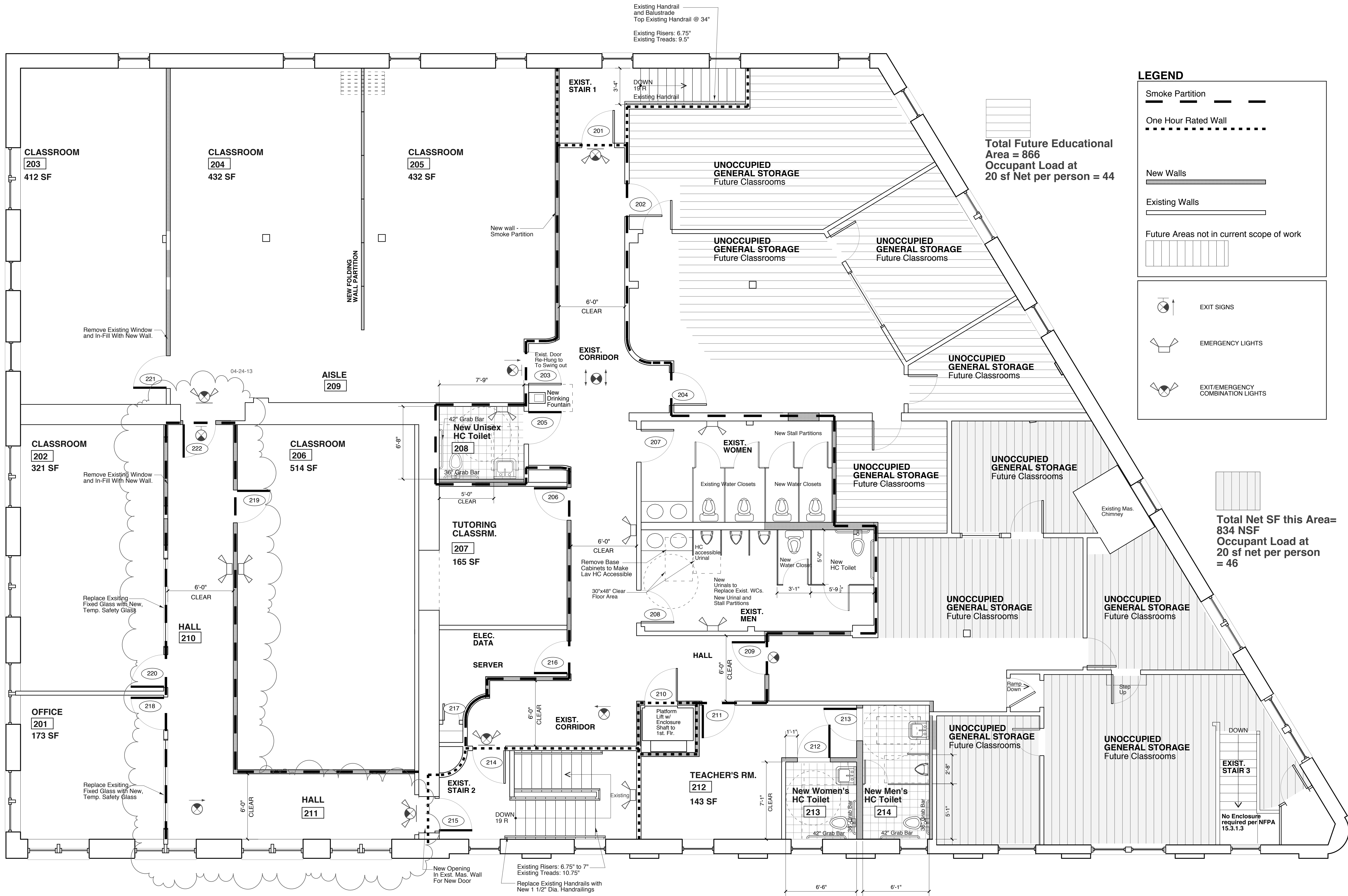
1 Second Floor Plan SCALE: 1/4"=1'-0"
