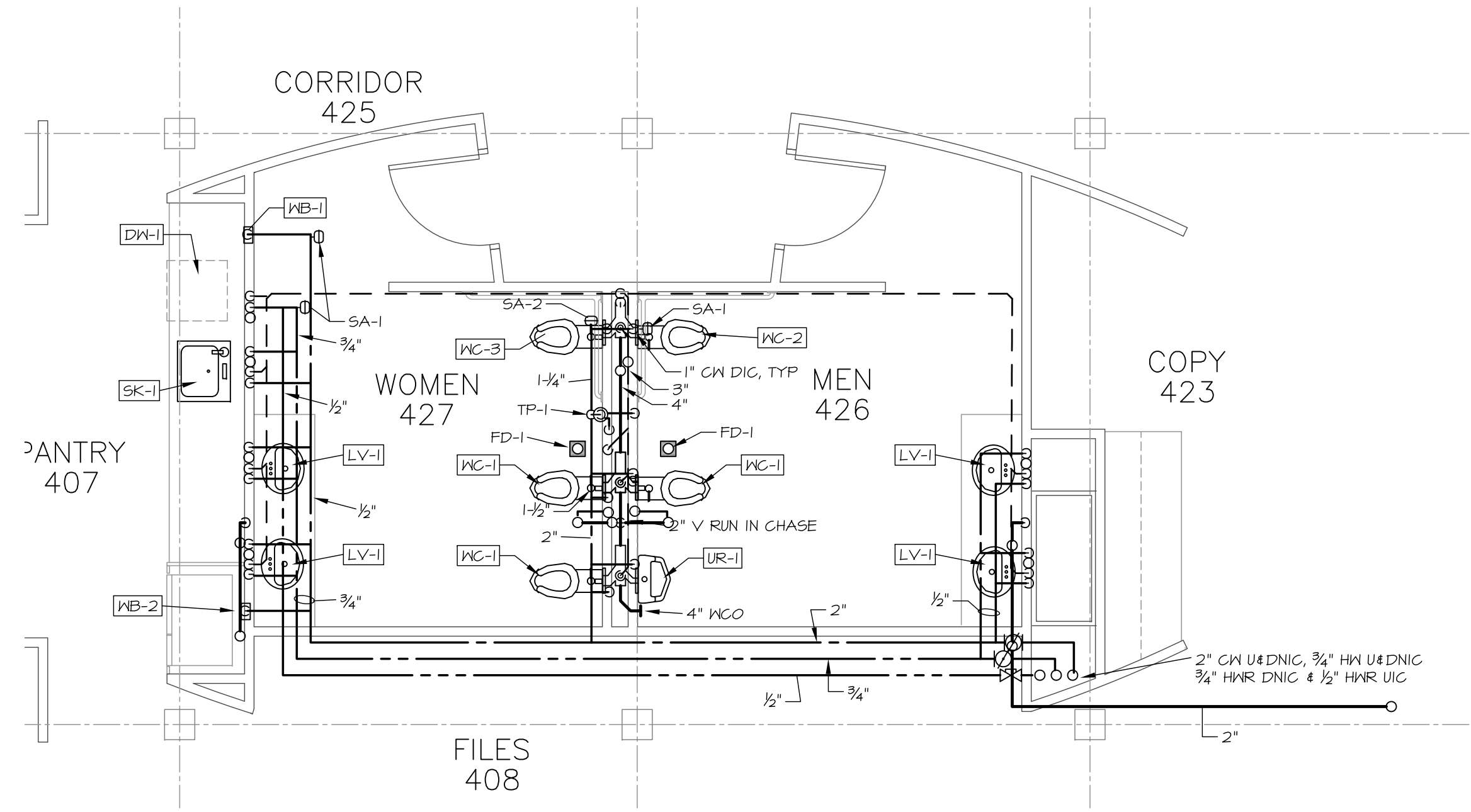
GROUP BATHROOMS PLUMBING PLAN SCALE: 1/4" = 1'-0"
