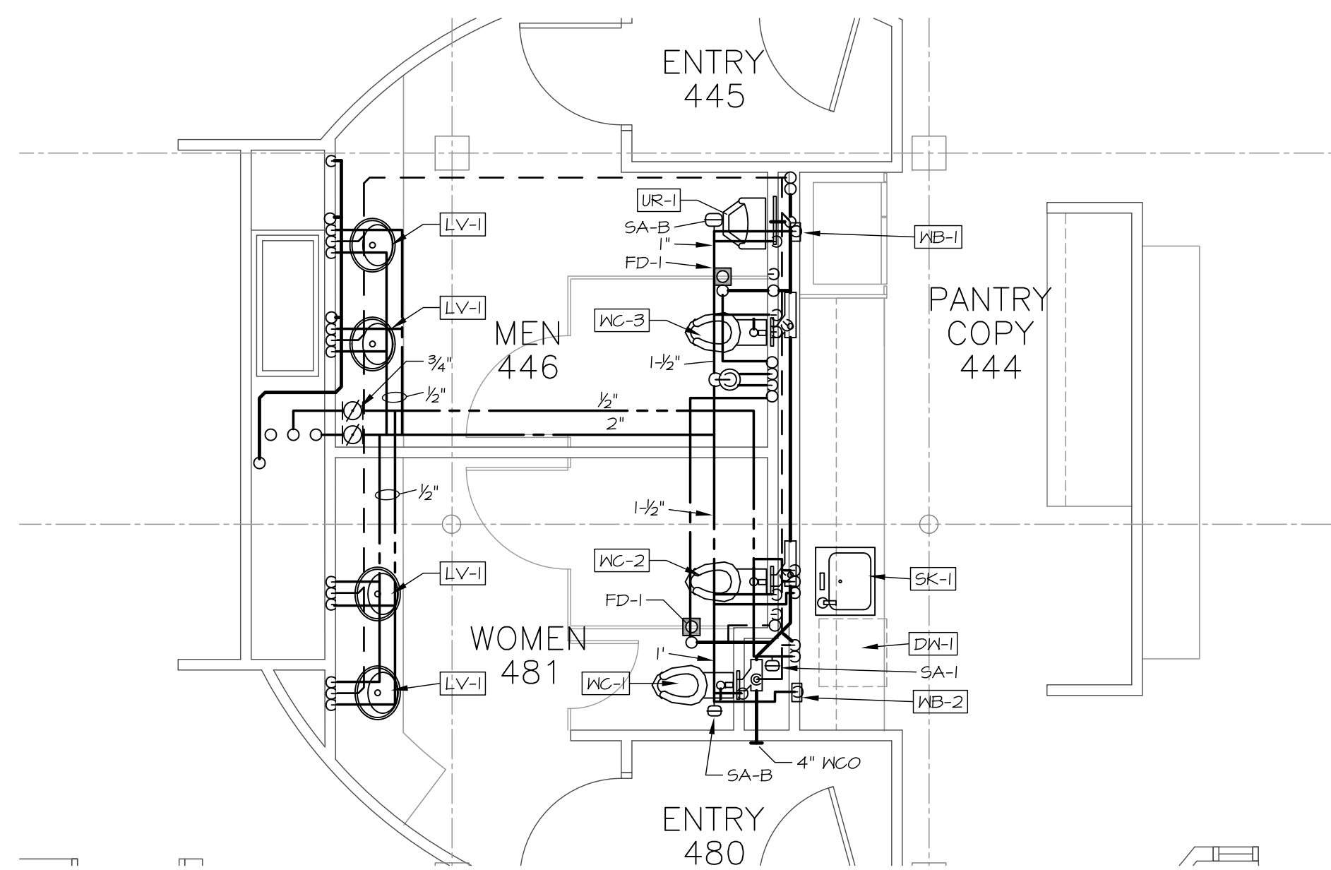
GROUP BATHROOMS PLUMBING PLAN SCALE: 1/4" = 1'-0"
