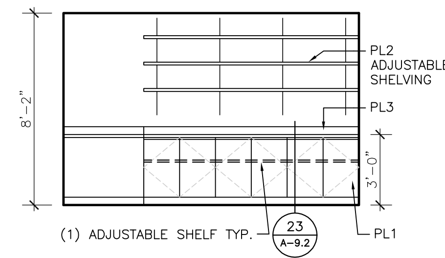
18 IT ROOM 438 1/4" = 1'-0"
