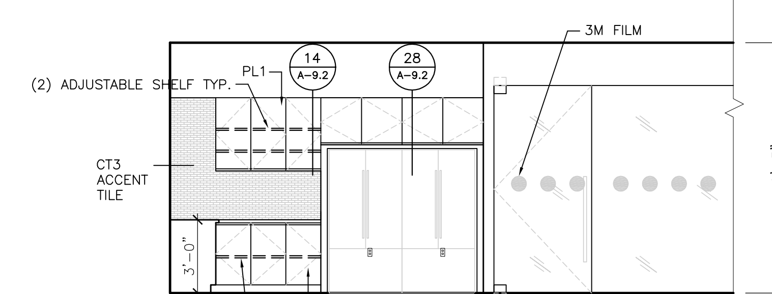
29 LOUNGE 545 1/4" = 1'-0"
