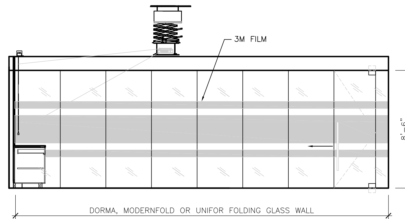
25 BOARD ROOM #506 1/4" = 1'-0"
