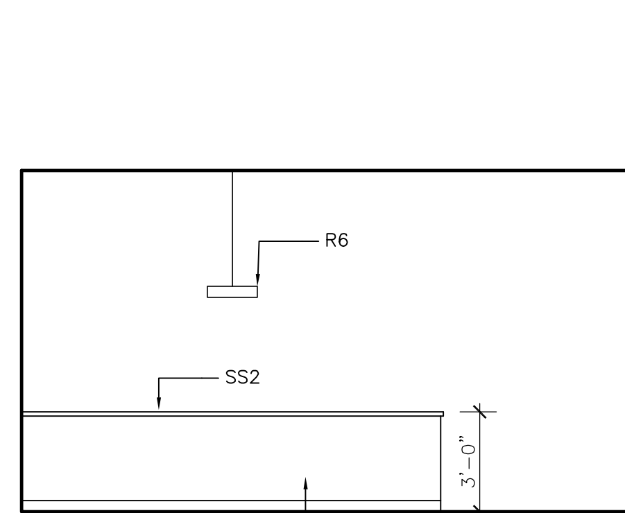
25 BOARD ROOM #506 1/4" = 1'-0"
