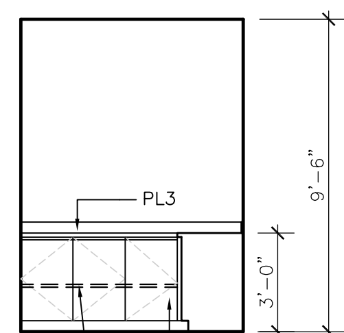
29 SERVERY 513 1/4" = 1'-0"
