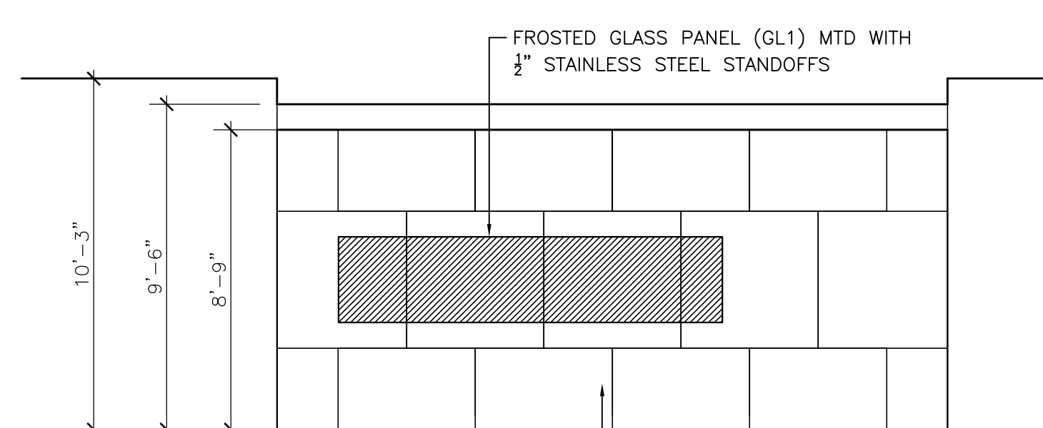
33 FLOOR 5 ELEVATOR LOBBY 1/4" = 1'-0"
