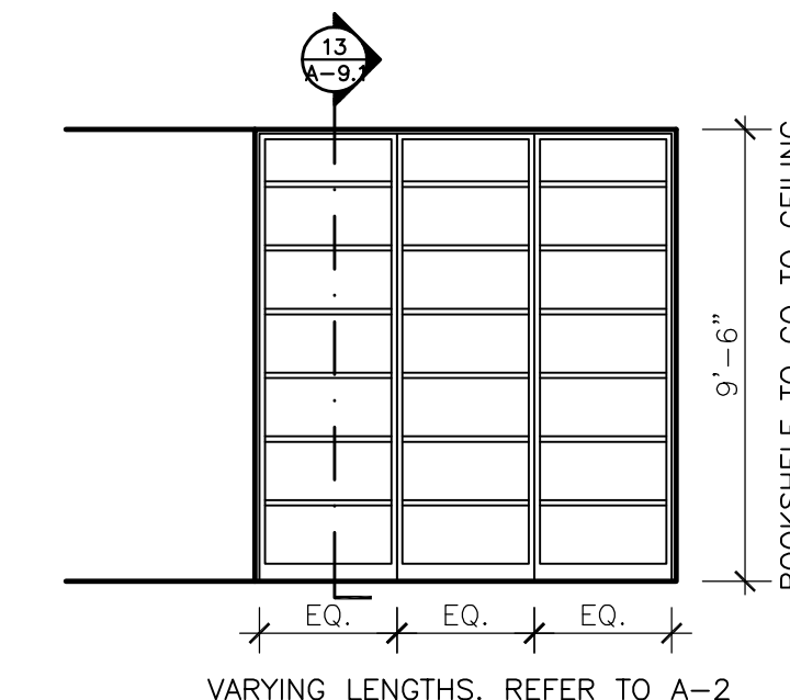
22 TYPICAL CONFERENCE CENTER BOOKSHELVES 1/4" = 1'-0"
