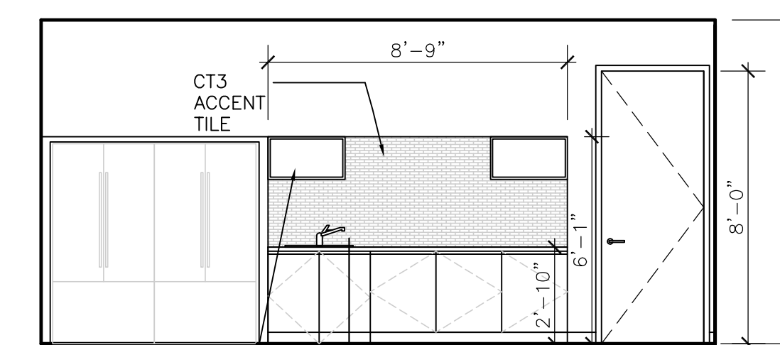
31 LOUNGE 545 1/4" = 1'-0"
