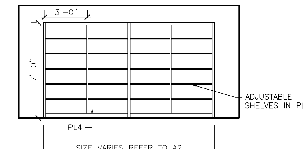
21 TYPICAL WAR ROOM BOOKSHELVES 1/4" = 1'-0"
