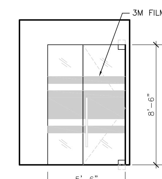
27 PHONE ROOM 535 1/4" = 1'-0"
