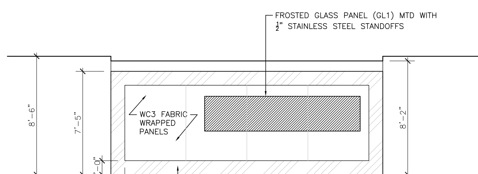
34 FLOOR 2,3,4 ELEVATOR LOBBY 1/4" = 1'-0"
