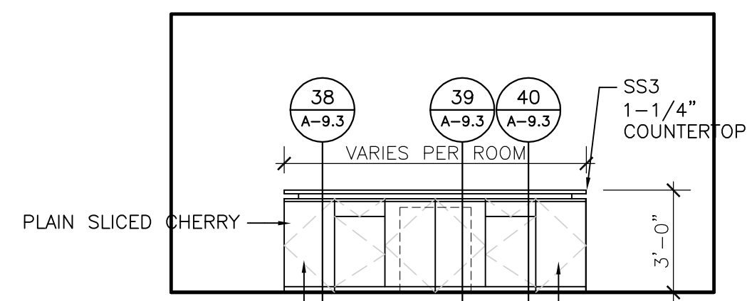
24 TYPICAL CONFERENCE ROOM LARGE CREDEZZA 1/4" = 1'-0"
