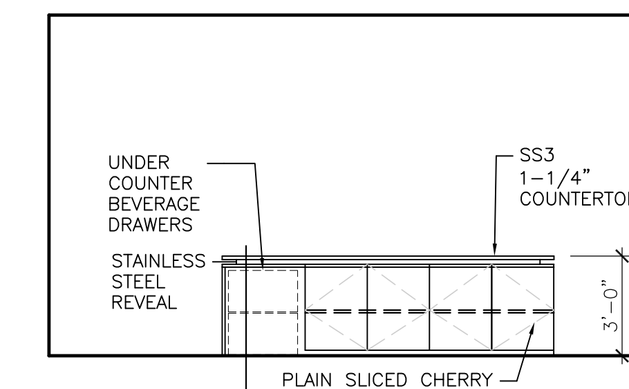
26 CONFERENCE CENTER ISLAND 1/4" = 1'-0"
