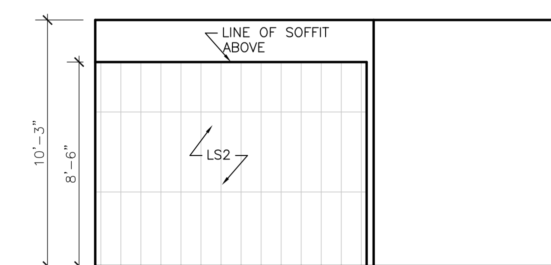
35 RECEPTION 502 1/4" = 1'-0"
