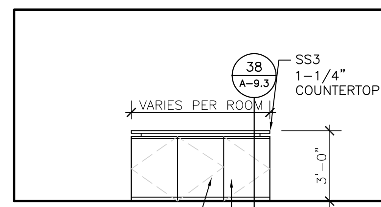
23 TYPICAL CONFERENCE ROOM SMALL CREDEZZA 1/4" = 1'-0"
