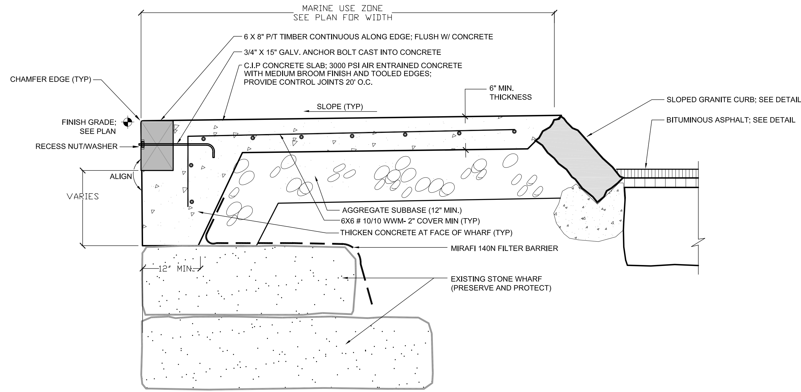
1 WHARF DECK-TYPICAL SECTION NOT TO SCALE
