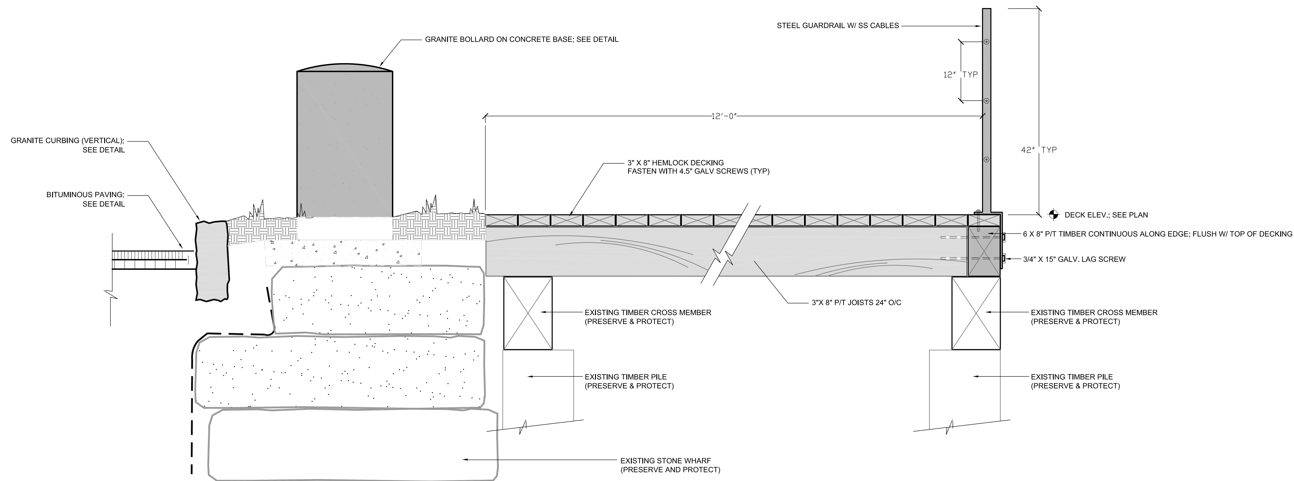
2 WOOD DECK-TYPICAL SECTION NOT TO SCALE
