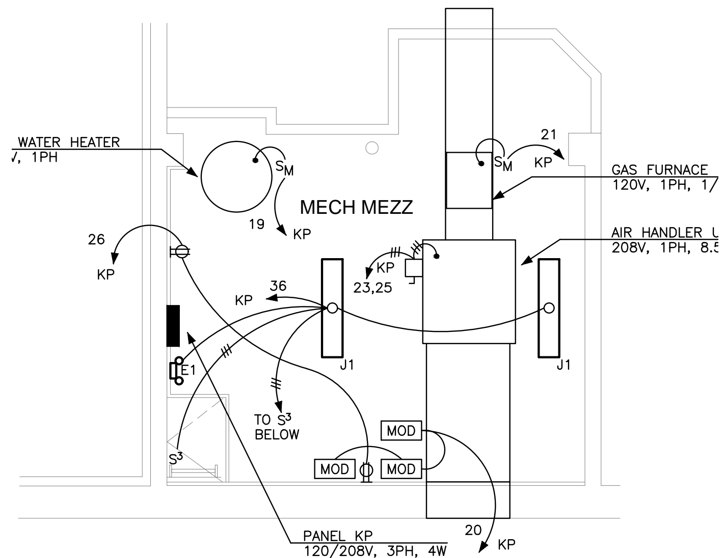
MECHANICAL MEZZANINE 1/4" = 1'-0"
