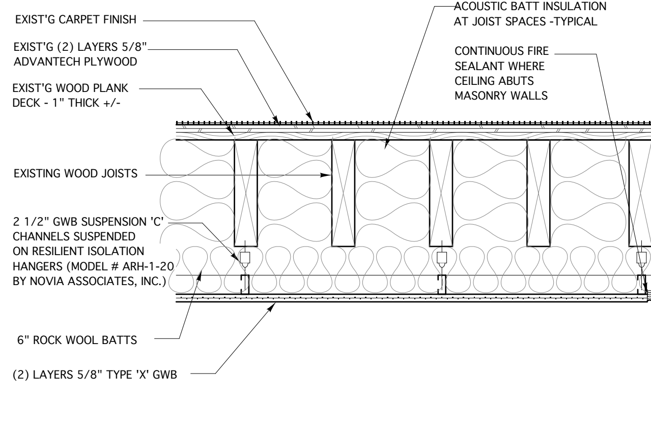
C2 CEILING ASSEMBLY DETAIL - 1 HOUR RATED 3/4" = 1'-0"
