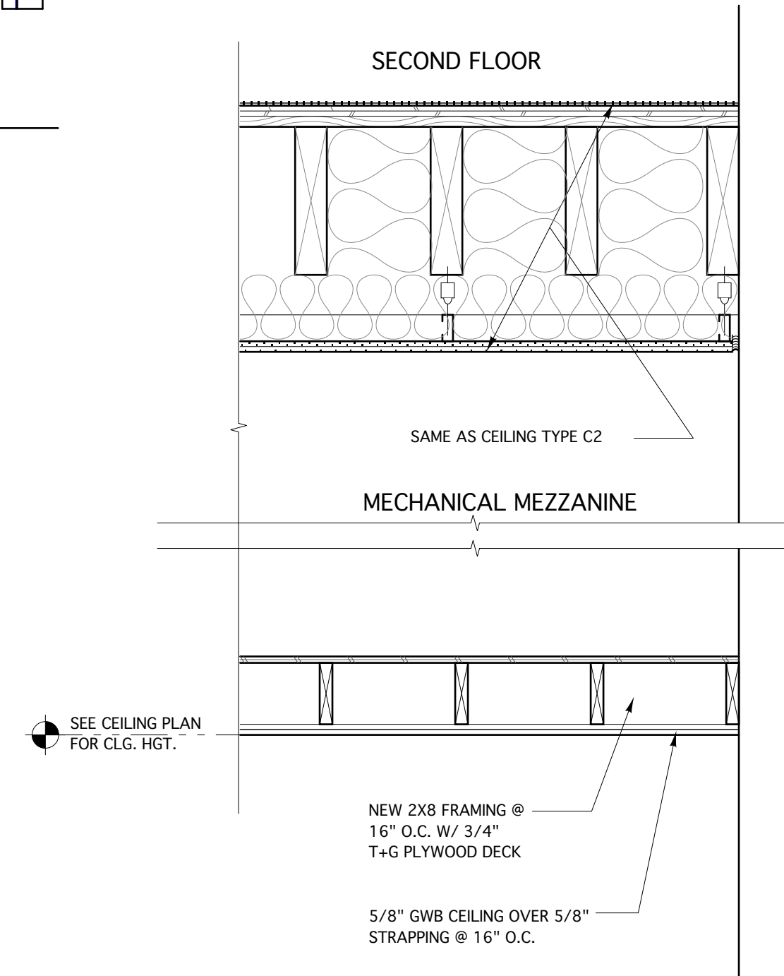
C3 CEILING ASSEMBLY DETAIL - 1 HOUR RATED 3/4" = 1'-0"
