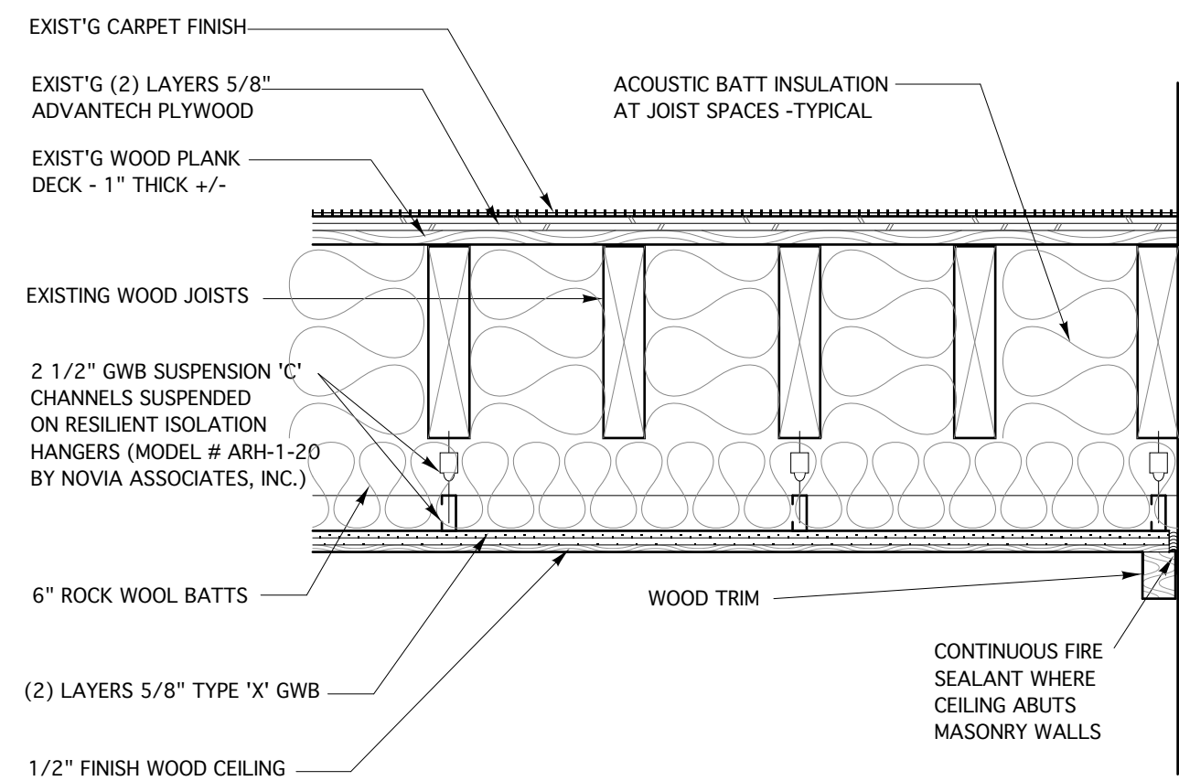
C1 CEILING ASSEMBLY DETAIL - 1 HOUR RATED 3/4" = 1'-0"
