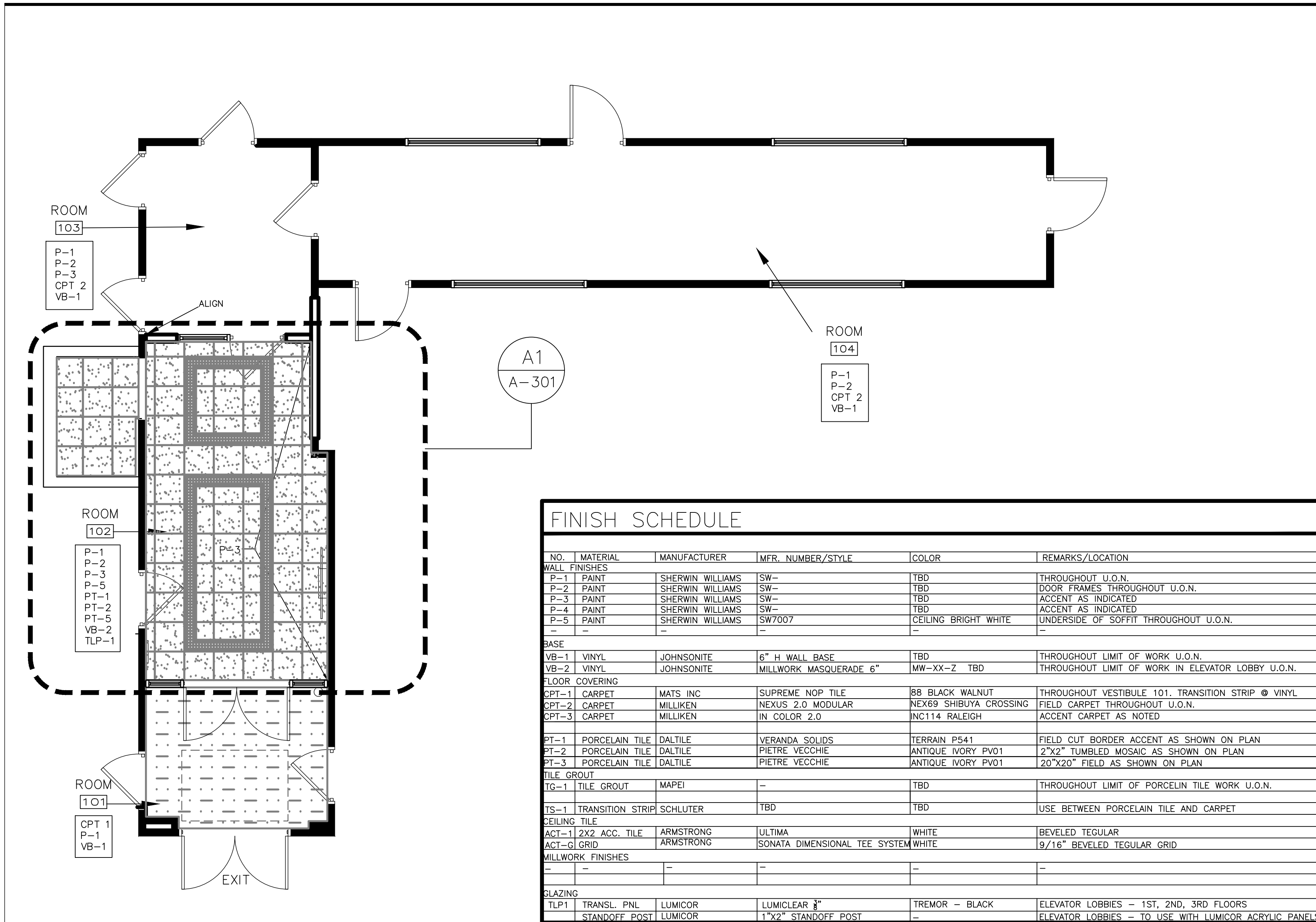
A2 FINISH PLAN - 1ST FLOOR 1/4" = 1'-0"
