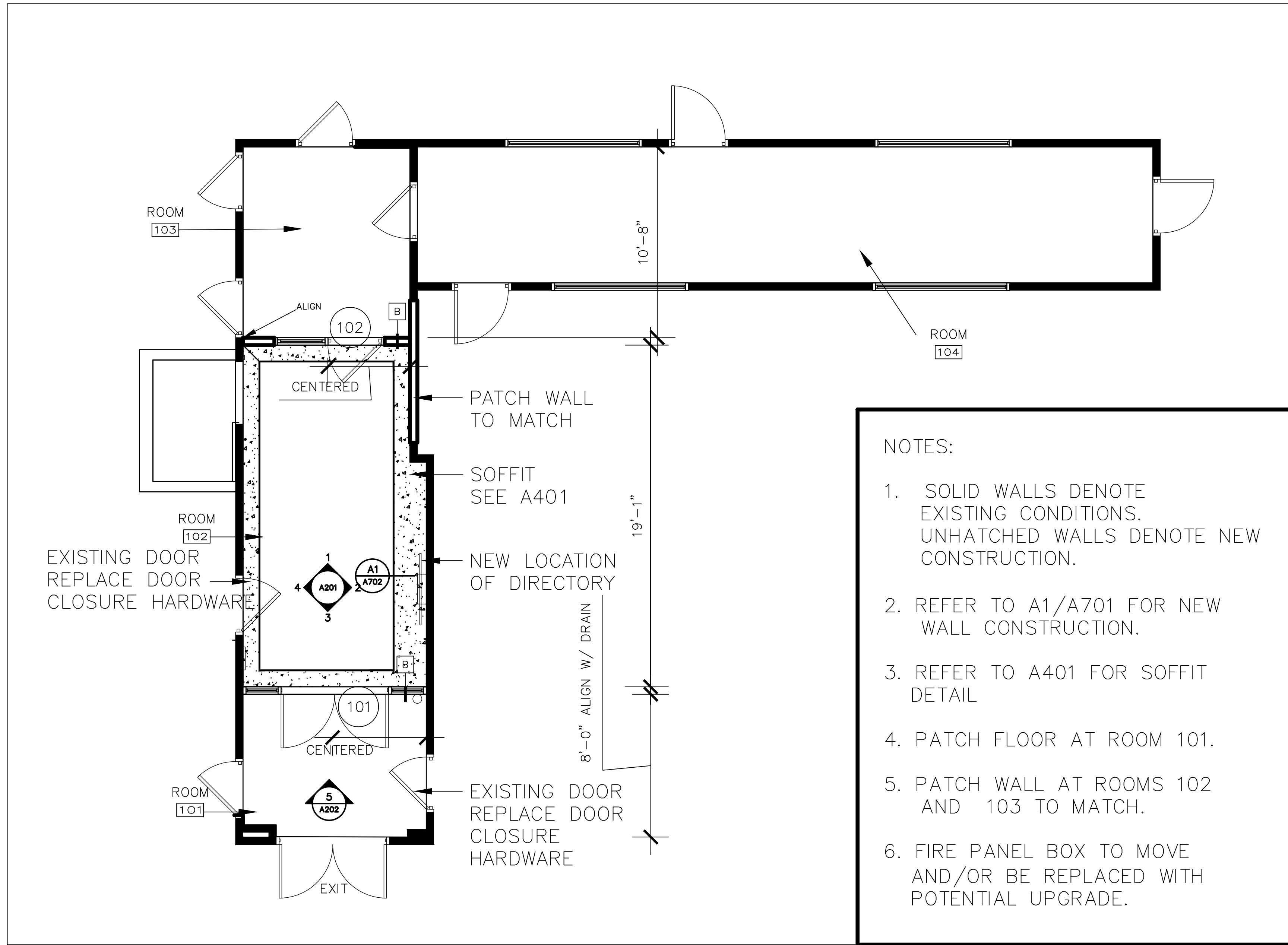
(A1) 1ST FLOOR CONSTRUCTION PLAN 1/4" = 1'-0"
