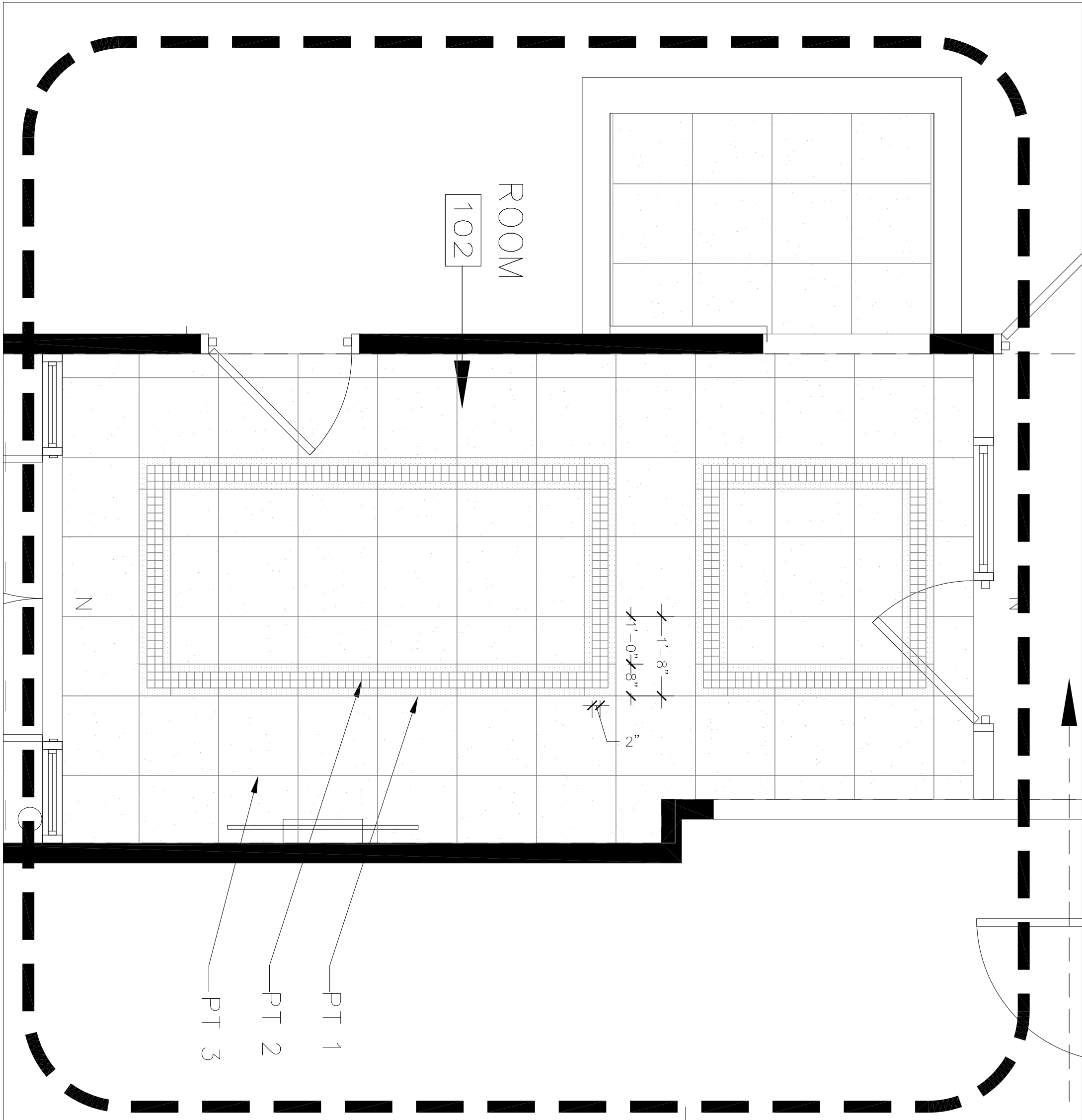
A1 ENLARGED PARTIAL PLAN - 1ST FLOOR 1/2" = 1'-0"
