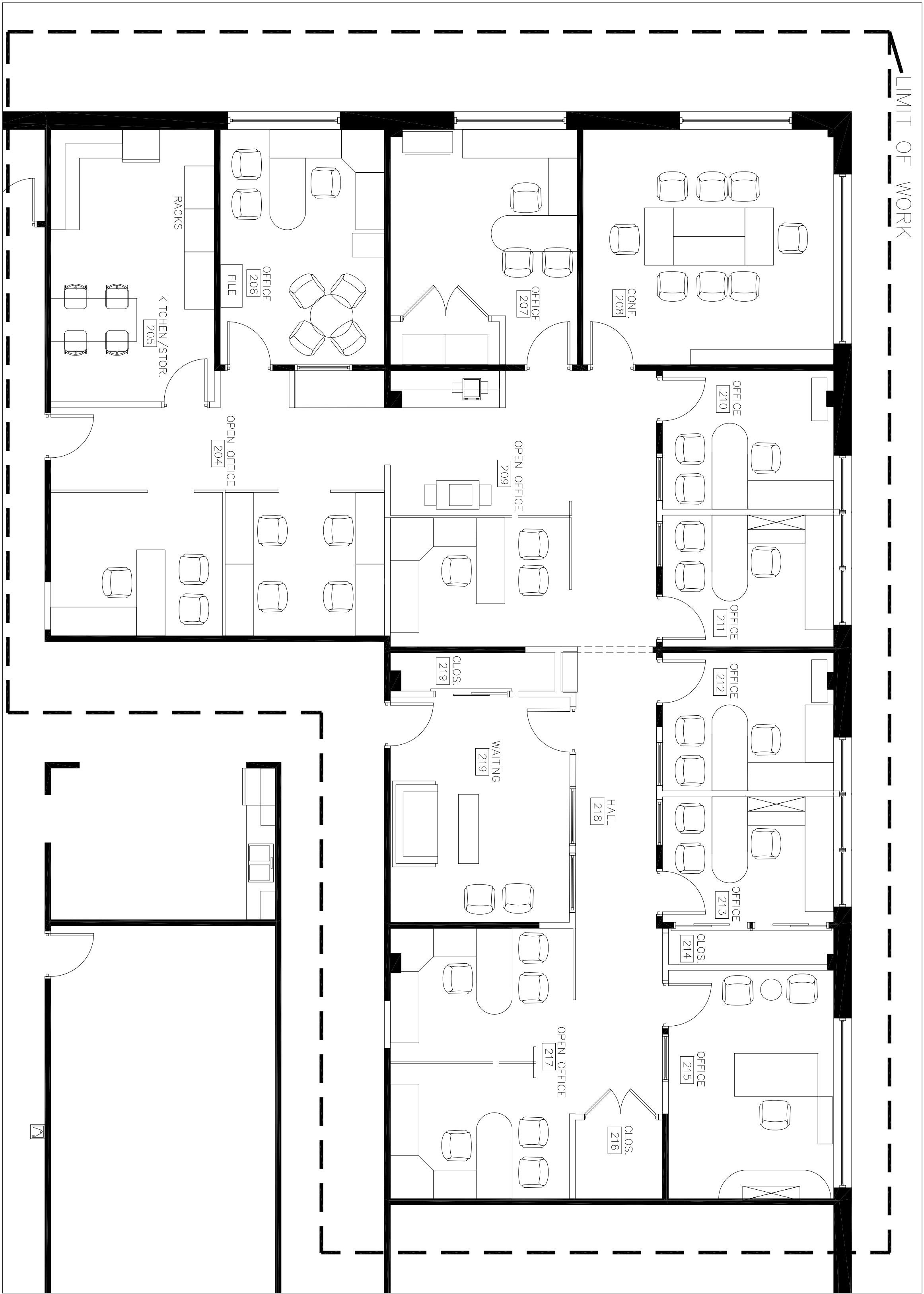
A1 2ND FLOOR FURNITURE & EQUIPMENT PLAN 3/16" = 1'-0"
