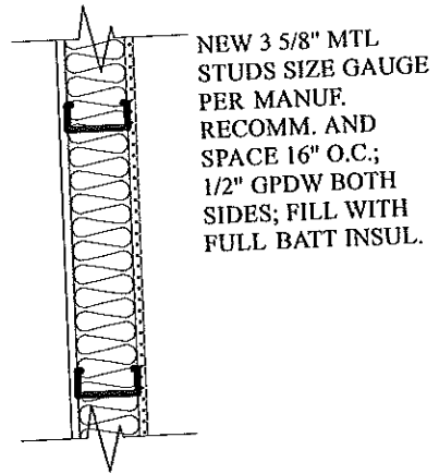
X TYPICAL ALL INTERIOR PARTITIONS U.O.N.
