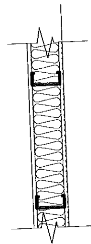
1HR 1 HOUR FIRE RATED PARTITION
