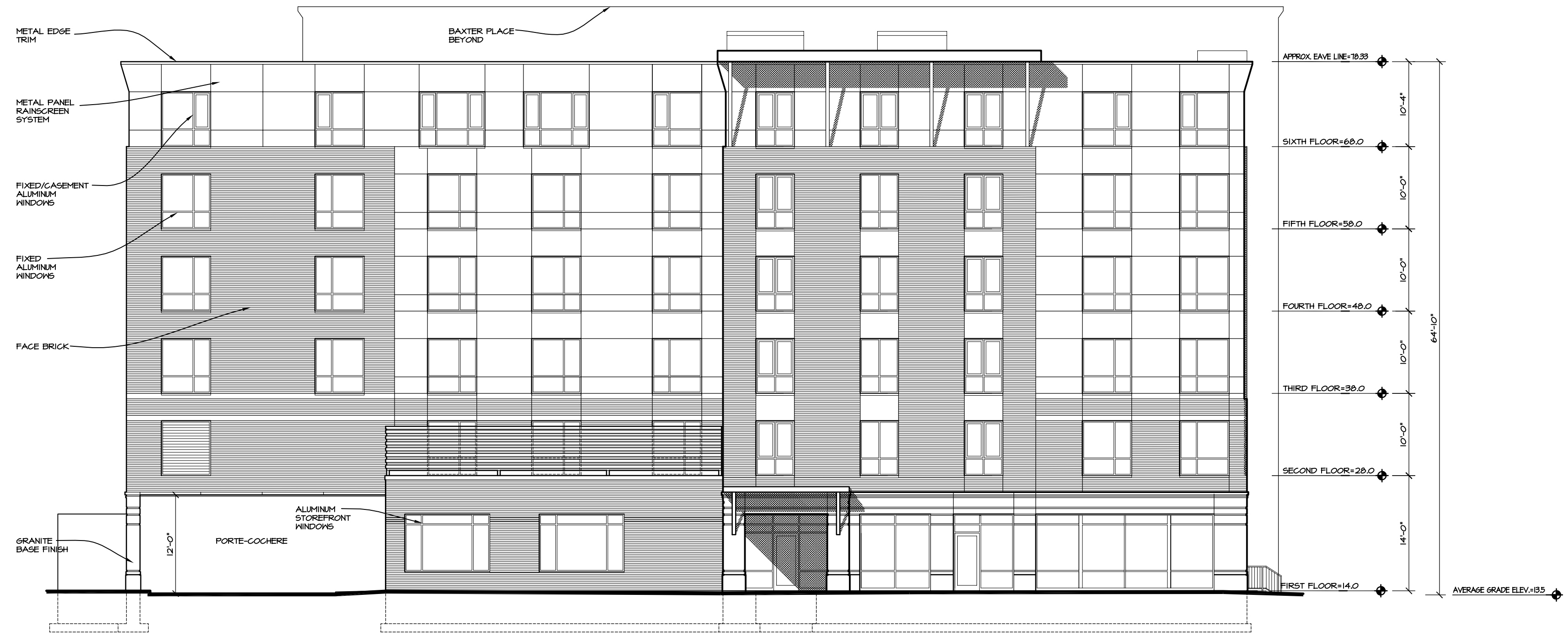
1 MAPLE STREET ELEVATION C12 3/32" = 1'-0"
