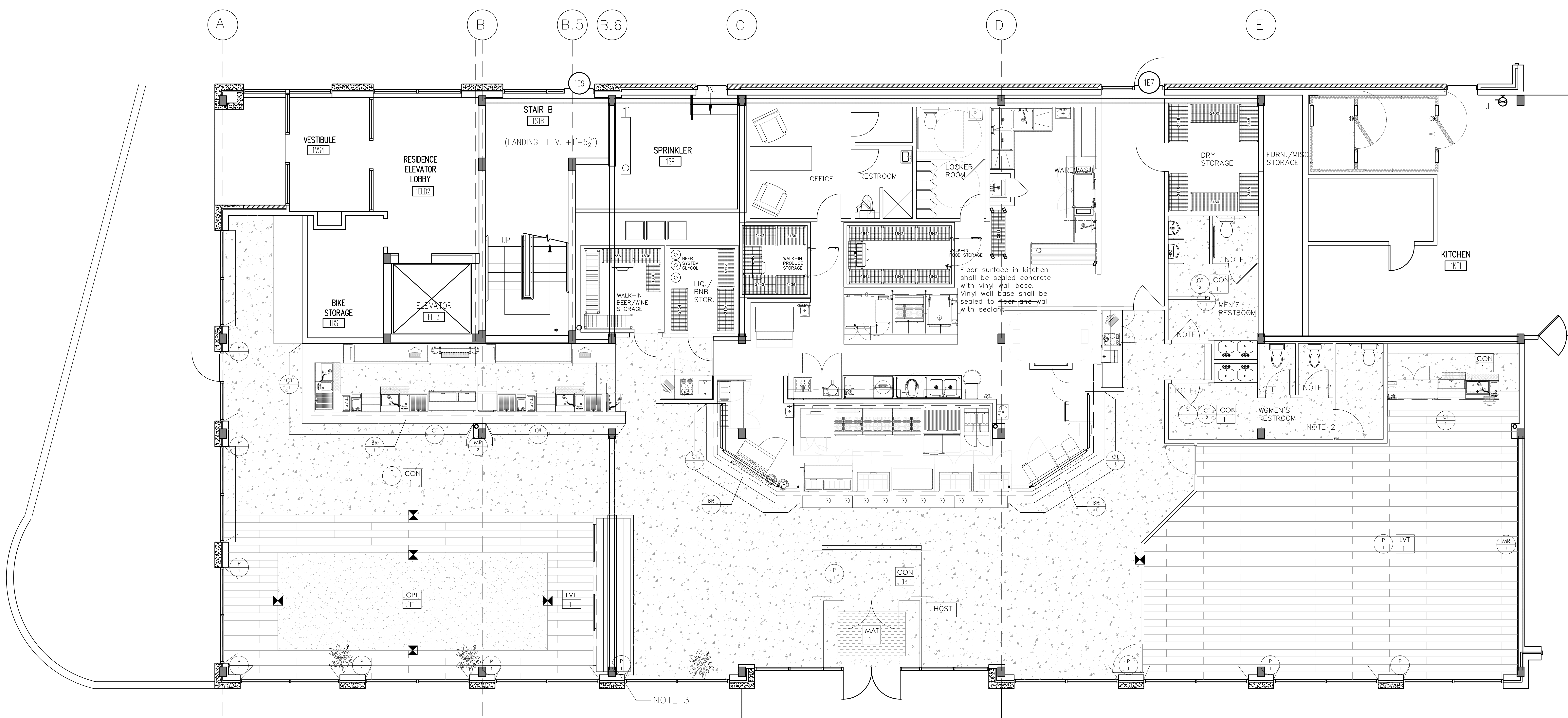
1 GROUND FLOOR FINISH PLAN
