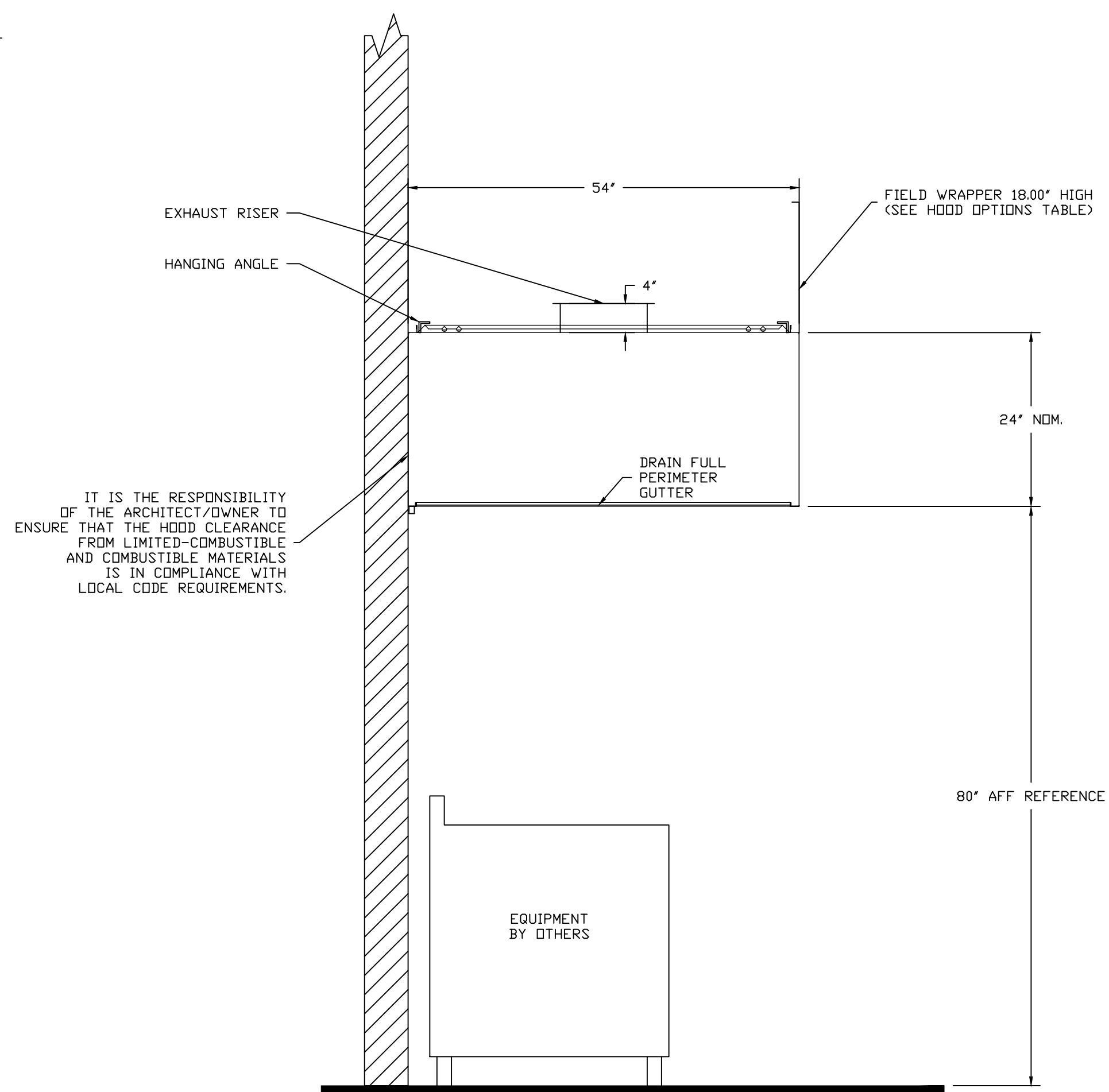
SECTION VIEW - MODEL 5424VHB-G HOOD - #4 (Dish)
