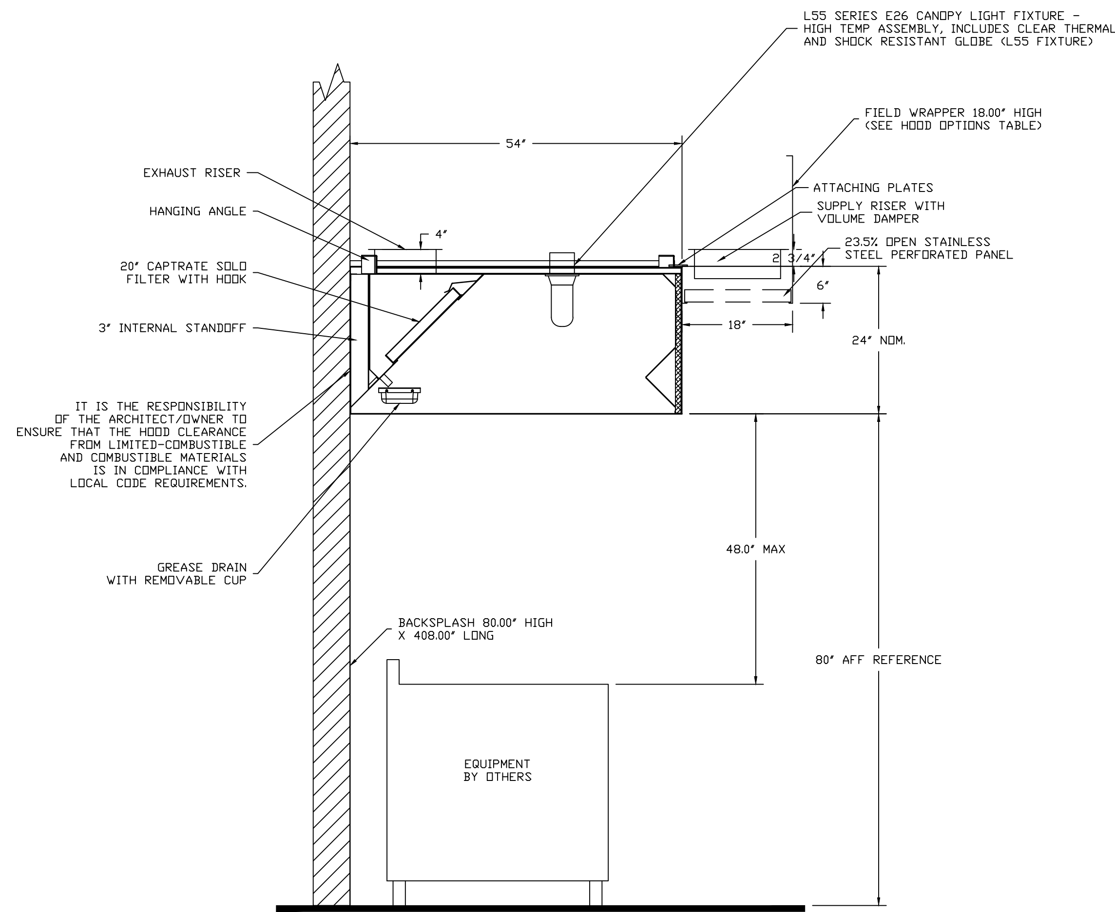
SECTION VIEW - MODEL 5424ND-2-PSP-F HOODS - #1 (Left), #2 (Right), #3
