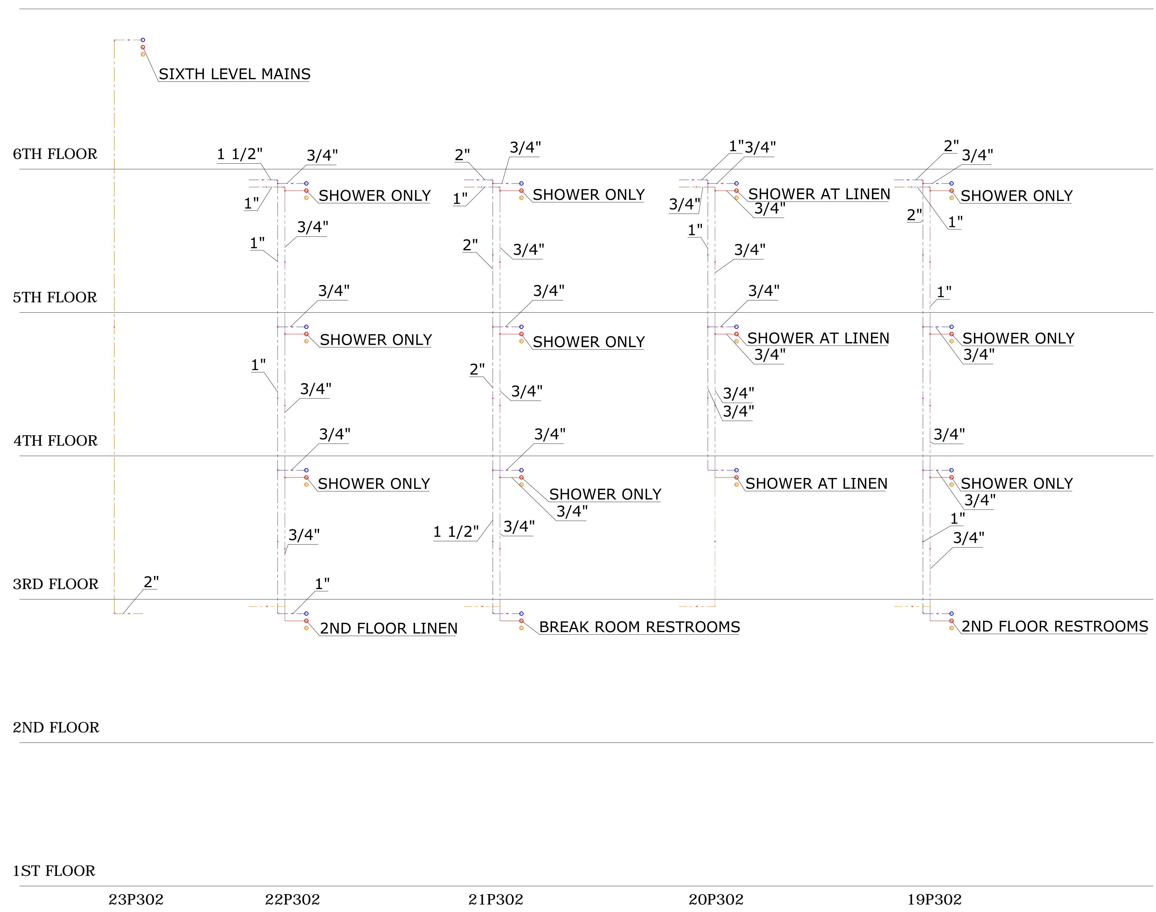
19-23 P302 TYPICAL RISERS 1/4" = 1'-0"
