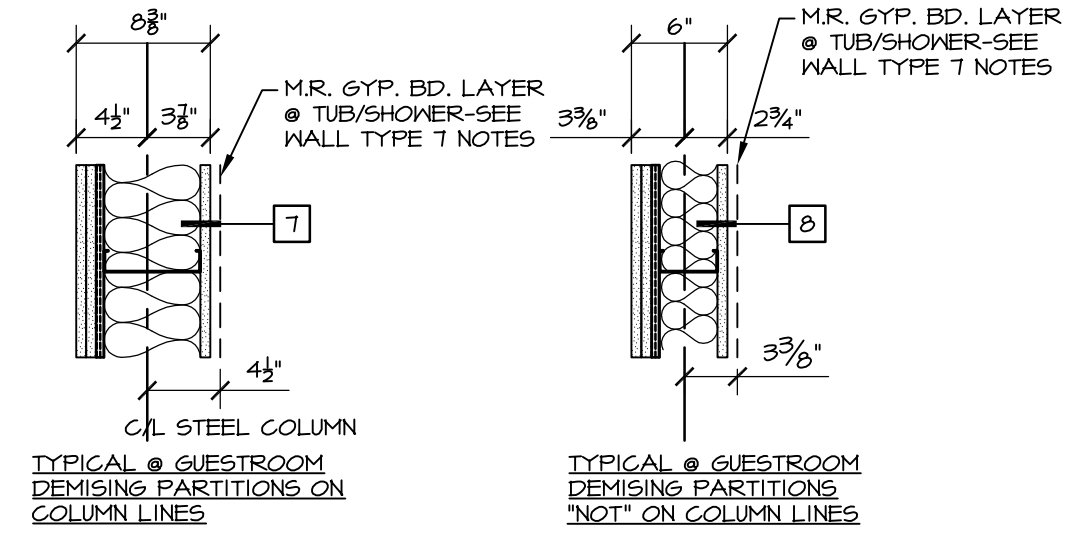
GUESTROOM DEMISING WALL LOCATIONS 1" = 1'-0"
