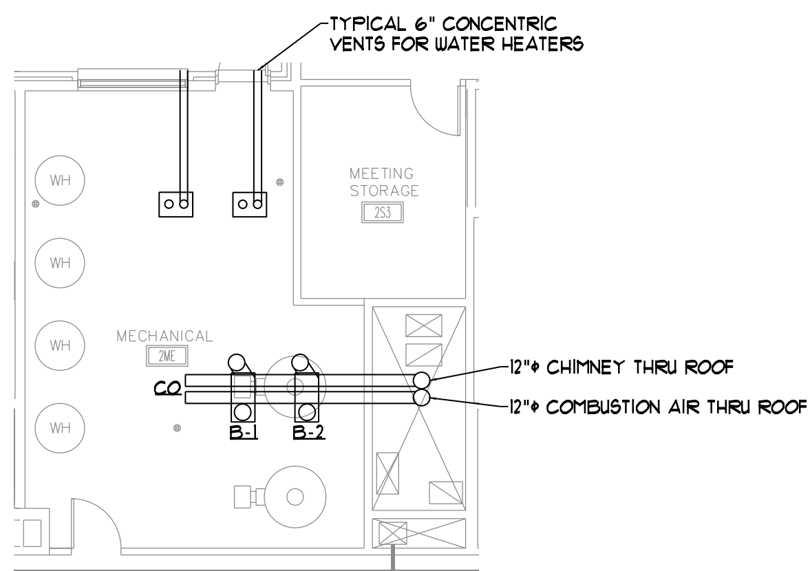
MECHANICAL ROOM PART PLAN SCALE: 1/8" = 1'-0"
